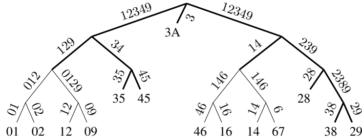
Fig. 4: A branch decomposition \mathcal{B} of the graph H given in Fig. 3 together with an example of a local branch decomposition \mathcal{B}_L (highlighted by thicker edges) chosen by our algorithm.
