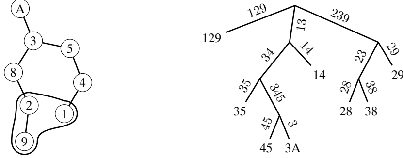
Fig. 1: A hypergraph H (left) and an optimal branch decomposition (T, \gamma) of H (right). The labels of the leaves of T are the edges assigned to them by \gamma and the labels of the edges of T are the load vertices of that edge.
