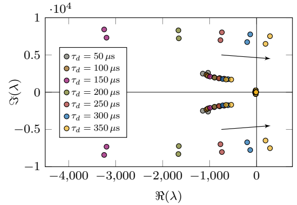
Fig. 5: Root loci spectrum around the imaginary axis computed using the Padé approximation.
