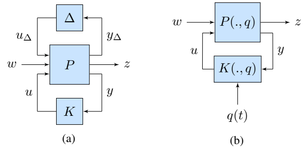
Fig. 2: General control plant: (a) LFT general plant. (b) LPV general plant.
