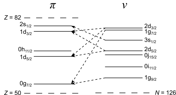
Fig. 1. Shell model orbitals for 50 < Z < 82 and 126 < N < 184 . The ordering and energy spacing of the orbitals are taken from the experimental level schemes of ^{207}\text{Tl} and ^{209}\text{Pb} respectively [4]. Arrows link proton-neutron pairs which satisfy the \Delta I = 0, \Delta n = 1 condition.
