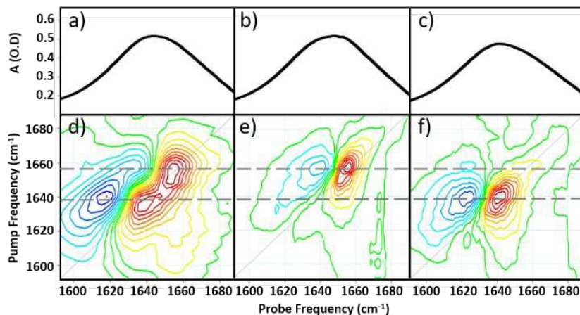
Figure 3. IR absorption spectra of (a) serum (b) serum albumin (c) \gamma -globulins. 2D-IR spectra of (d) serum (e) serum albumin (f) \gamma -globulins. Dashed grey horizontal lines show peak positions of albumin and \gamma -globulins. The color scale is as shown in Fig.2.
