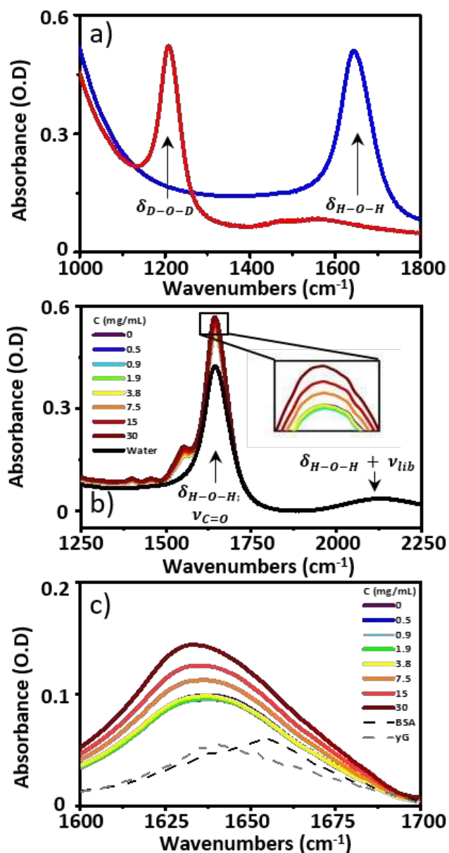
Figure 1: (a) The IR absorption spectra of D 2 O (red) and H 2 O (blue). (b) IR absorption spectra of serum samples spiked with \gamma -globulins, pure H 2 O is shown in black. The inset shows an expansion of the tip of the peak due to the H-O-H bending mode of water and the protein amide I band at 1650 cm -1 (c) IR absorption spectra of serum spiked with \gamma -globulins from (b) following subtraction of the H 2 O spectrum.
