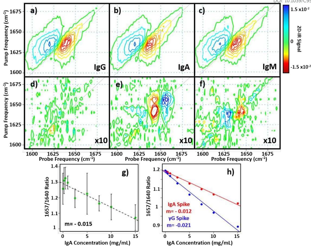
Figure 6: a-c) 2D-IR spectra of IgG, IgA and IgM in H 2 O. d-f) Difference spectra obtained by subtracting the 2D-IR response of the spectra in a-c) from that of the \gamma -globulins. The spectral features have been magnified by a factor of 10 for clarity and are shown on the same scale as a-c). g&h) show the variation in 2D-IR signal at the peak of the difference spectral response for IgA as a function of added protein for the experimental data (g) and simulations (h). The linear increase in the negative signal shows a correlation with protein content.
