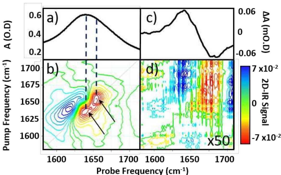
Figure 2. (a) IR absorption and (b) 2D-IR spectrum of pure serum in the amide I region. Arrows identify two components of the \nu=0-1 transition discussed in the text. (c) IR pump-probe spectrum of \text{H}_2\text{O} at a pump-probe time delay of 300 fs. (d) 2D-IR spectrum of \text{H}_2\text{O} , magnified 50x. The spectra in (b) and (d) were both obtained with a waiting time ( T_w ) of 250 fs and are plotted on the same scale, see colour bar.
