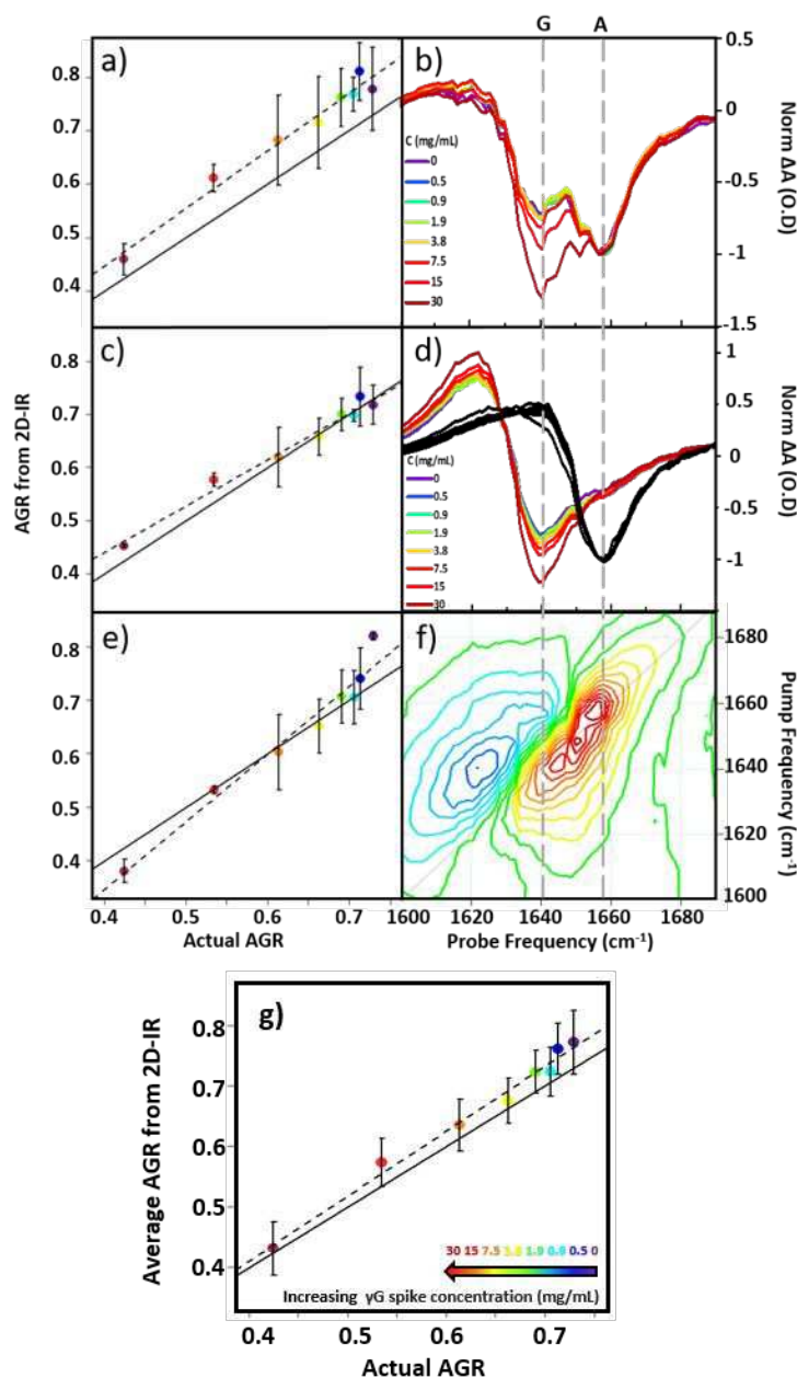
Figure 5: AGR of serum samples from 2D-IR spectroscopy. a&b) AGR obtained using the 2D-IR diagonal method. c&d) AGR obtained using the pump slice method. e&f) AGR values obtained using the 2D-IR linear combination method. The spectral basis of the method is shown in b), d) and f) respectively. g) AGR obtained from averaging the results in a), c) and e). In panels a), c), e) and g) the solid black line indicates the actual AGR of the samples. Error bars show 2σ variation. Dashed lines show linear fits to the experimental AGR values.
