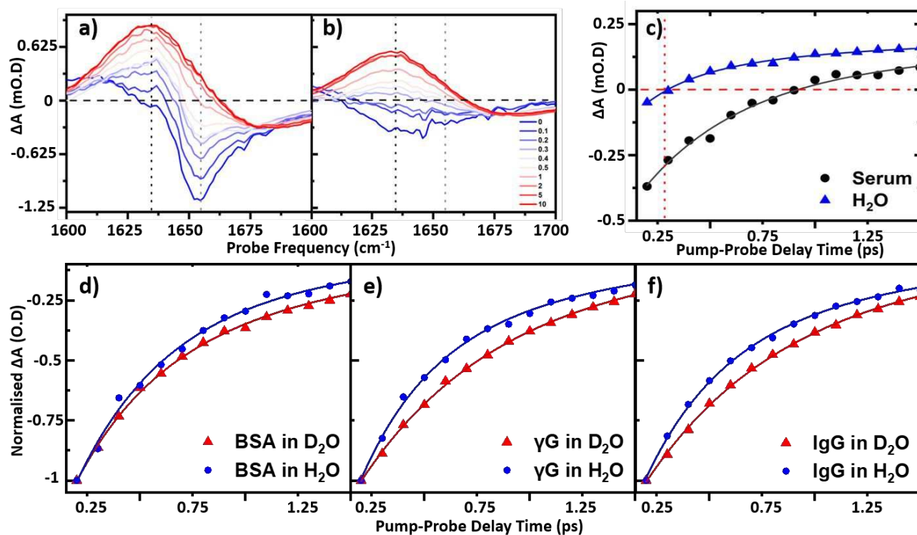
Figure 4. IR pump-probe spectra of (a) serum albumin and (b) \text{H}_2\text{O} . Waiting times range from 0 ps (blue) to 10 ps (red). (c) Temporal variation of the bleach signal observed in the IR pump-probe spectrum of \text{H}_2\text{O} (blue) and serum (black) at a frequency of 1650 \text{cm}^{-1} . Solid lines show fits to the data using a single exponential function with a decay time constant of 220 fs ( \text{H}_2\text{O} ) and 0.83 ps (serum) respectively. Temporal variation of the amide I v=0-1 bleach signal for (d) serum albumin (e) \gamma -globulins and (f) IgG in both \text{D}_2\text{O} (red) and \text{H}_2\text{O} (blue) solvents. All pump probe data were obtained with magic angle polarization of pump and probe pulses.
