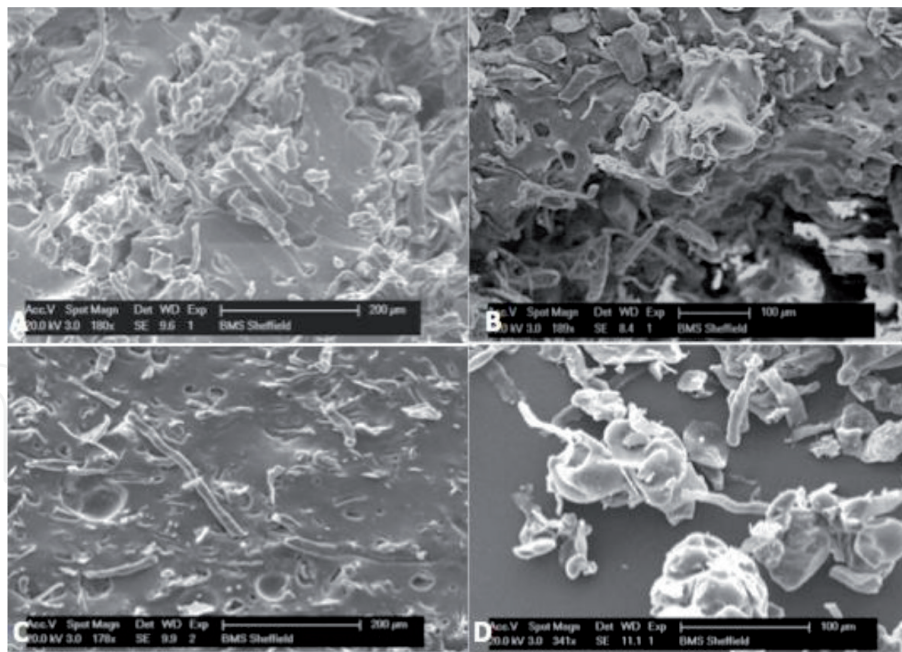
Figure 11. SEM for (A) 3D printed starch block infiltrated Sil-25 SP ( \times 180 ), (B) 3D printed starch block infiltrated Promax10 ( \times 189 ), (C) hand mixed starch powder and Sil-25 SP ( \times 178 ), (D) starch powder particles ( \times 341 ).
