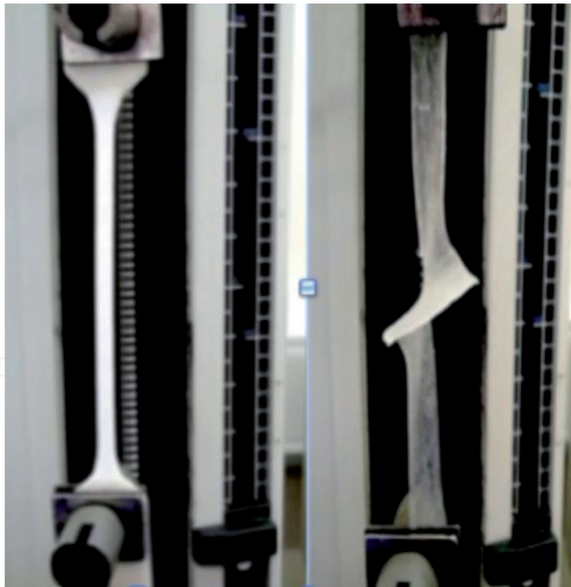
Figure 5. Lloyd LRX tensile tester testing tensile and tear strength of the printed samples.
