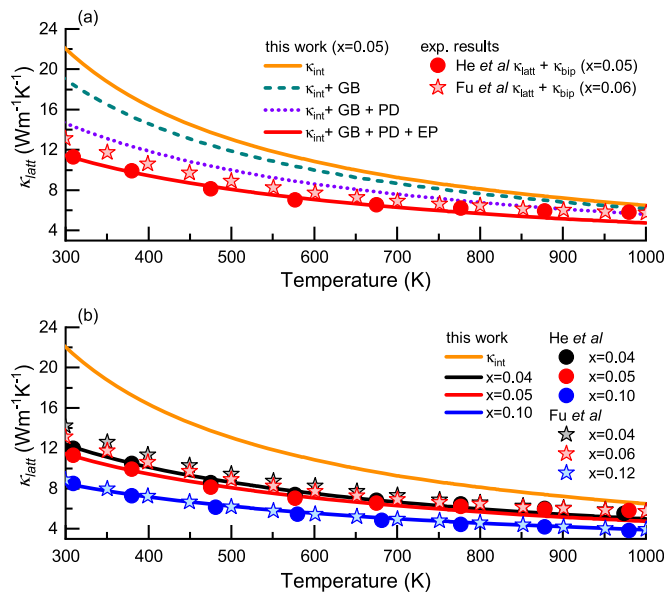
Figure 5. Figure (a) shows the contribution of grain boundaries GB, point defects PD and electron–phonon interaction EP to the lattice thermal conductivity \kappa_{latt} of NbFeSb. Figure (b) compares the theoretical prediction of this study (solid lines) for Nb 1-x Ti x FeSb with L_{GB} = 0.5 \mu\text{m} to the experimental results (stars and circles).
