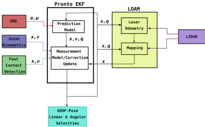
Fig. 2. The block diagram detailing an overview combination structure of the Pronto and LOAM algorithms. The estimation of the particular base state contributed to by the sensor or processing block is represented by the italic letters. The position is represented by x , the linear velocity by v , the acceleration by a , the angular velocity by \omega and the orientation quaternion by q .
