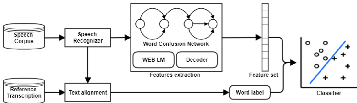
Figure 1: General workflow of the proposed approach.
