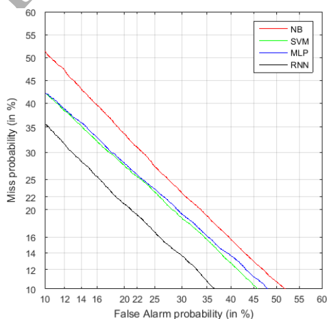
Figure 5: DET Plot comparing classifiers detection performance: BN, SVM, MLP and V-RNN on the test set using baseline feature set.
