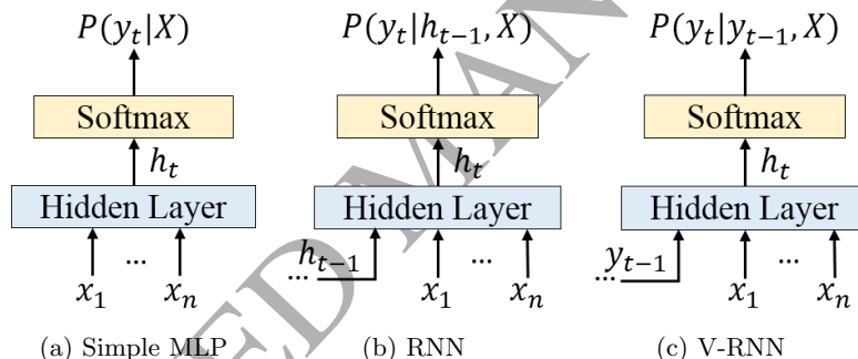
Figure 4: Neuronal based models for ASR error detection and classification
