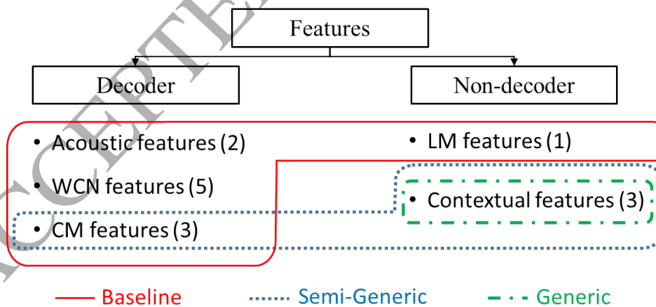
Figure 2: Features categorisation
