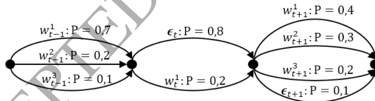
Figure 3: Sample Word Confusion Network.
