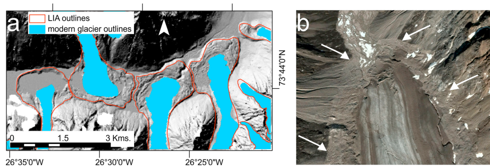
Figure 2. Examples of Little Ice Age (LIA) outlines mapped onto crest of outermost prominent moraine ridges on hill-shaded digital elevation model (a) and of depositional and erosional trimlines at Skillegletscher, Clavering Island, here in perspective view of Planet image (b).
