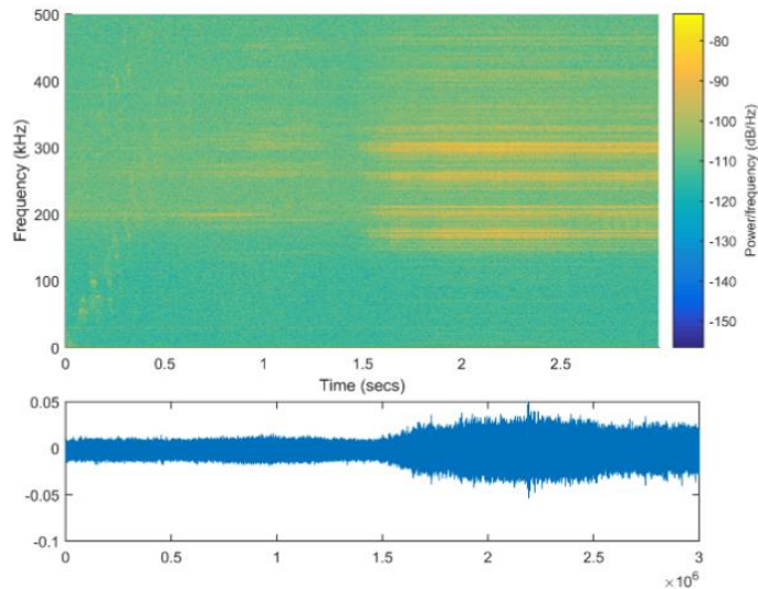
Figure 5: Opening flow scheduling valve response (Mills et al. 2018)
