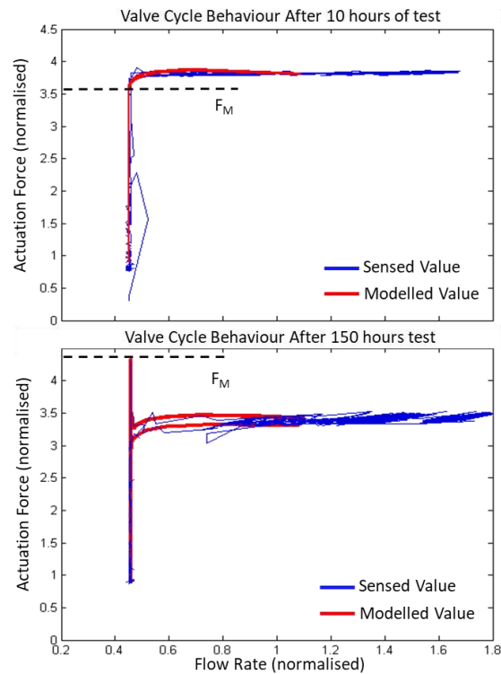
Figure 6: Valve actuation response to before and after fuel endurance testing on the AFTS rig (Mills et al. 2018).
