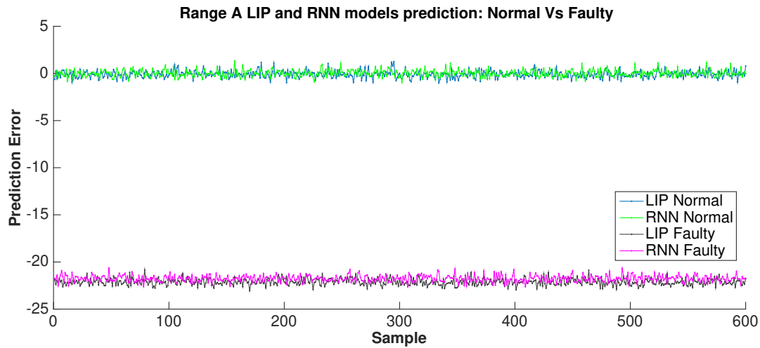
Figure 11: Prediction errors in normal and faulty condition (Fu et al. 2016)
