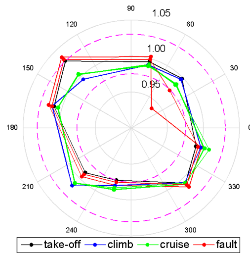
Figure 8 Radar plots of normalised T550 profiles (Fu et al. 2016)
