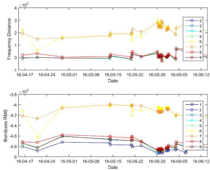
Figure 7: Acoustic spectrum features generated from data snapshots collected between April and June 2016, showing difference between open state (snapshots 6 & 7) and closed state (Mills et al. 2018)
