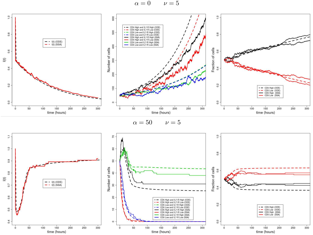
Figure 11: Numerical study for a total time of two weeks with high IL7 production, \nu = 5 for two values of \alpha : \alpha = 0 (top row) and \alpha = 50 (bottom row). On the left plot, we follow the extra-cellular IL7 concentration in time. On the middle plot, we follow the four cellular populations in time. On the right plot, we follow the two cellular populations, as defined by their CD5 expression in time.
