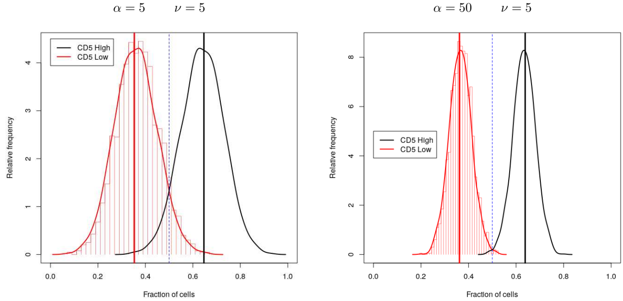
Figure 12: Histogram of the steady state of CD5 high subpopulation (black) and CD5 low subpopulation (red) for \nu = 5 and \alpha = 5 (left) or \alpha = 50 (right). The blue dashed vertical line is a guide to the eye to show the line where the fraction of each subpopulation is 50%.
