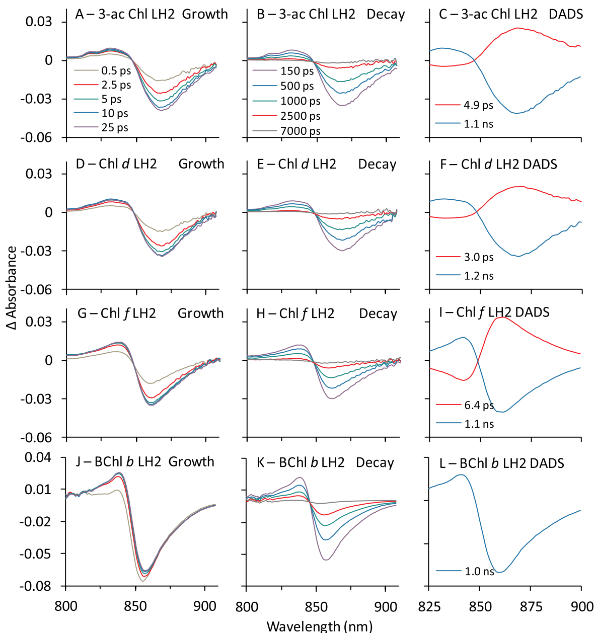
Fig. 7. NIR TA spectra during growth or B850* (left panels) and decay of B850* (centre panels), and DADS (right panels) for WT LH2 reconstituted with 3-acetyl Chl a (Panels A–C), Chl d (D–F), Chl f (G–I), and BChl b (J–L). Samples were excited at 690 (3-acetyl Chl a ), 700 (Chl d and Chl f ), and 820 nm (BChl b ).
