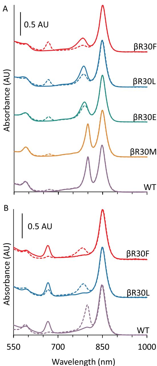
Fig. 4. A. Vis/NIR absorption spectra of WT (purple), \beta R30M (orange) \beta R30E (green) \beta R30L (blue) and \beta R30F (red) LH2 complexes either containing B800 BChl a (solid lines) or following incubation in five-fold excess of Chl a (dashed lines). B: Absorption of spectra of WT (purple), \beta R30L (blue) and \beta R30F (red) LH2 containing Chl a in the B800 site (solid lines) or following incubation in excess BChl a (dashed lines).
