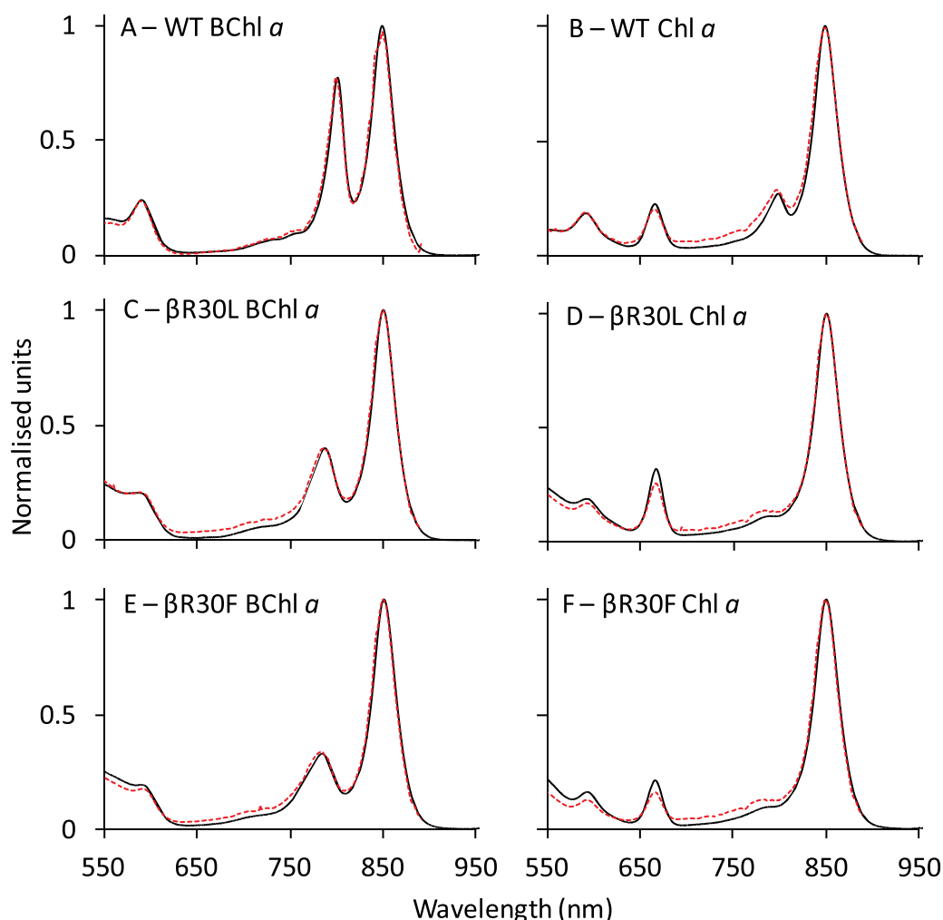
Fig. 8. Absorbance (1 – transmittance) (black) and fluorescence-excitation (red) spectra of (A) WT LH2 containing B800 BChl a , (B) WT LH2 containing B800 Chl a , (C) \beta R30L LH2 containing B800 BChl a , (D) \beta R30L LH2 containing B800 Chl a , (E) \beta R30F LH2 containing B800 BChl a , and (F) \beta R30F LH2 containing B800 Chl a . Excitation spectra were obtained using fluorescence detection between 890 and 900 nm. All spectra are normalised at 850 nm.
