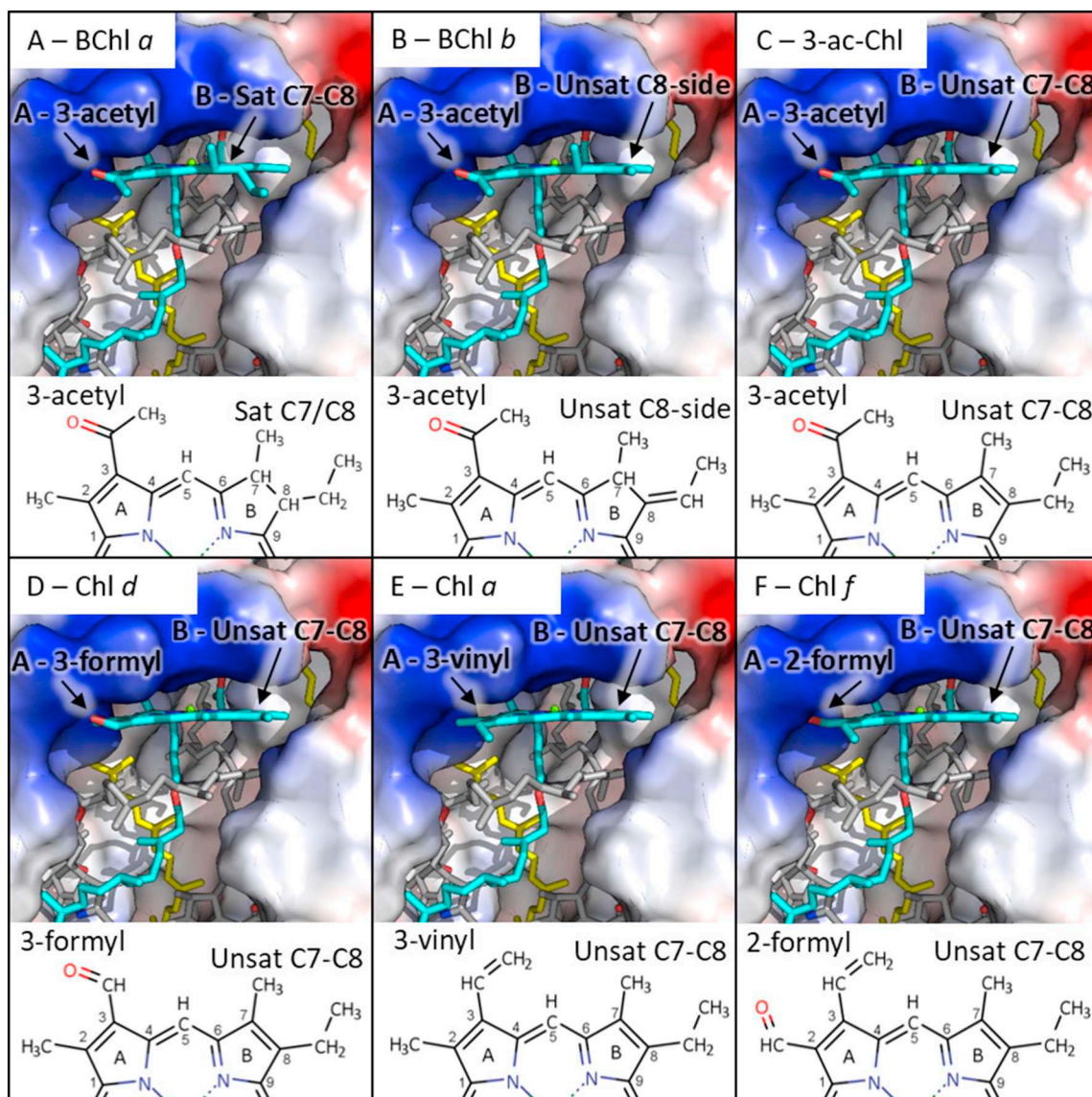
Fig. 2. Models of (B)Chls in the B800 site of Rbs. acidophilus LH2 (PDB ID: 1NKZ) [14]. The polypeptides are shown in surface representation with positive charges in blue, negative in red and uncharged regions in white. Cofactors are in stick representation with B850 in grey and carotenoid in yellow. The B800 BChl a has been coloured cyan (Panel A). Models of LH2 containing BChl b (Panel B), 3-acetyl Chl a (Panel C), Chl d (panel D), Chl a (Panel E), and Chl f (Panel F) in the B800 site are also shown. Below each structure are 2D representations of the A and B rings of each (B)Chl with rings A, B and carbons 1–9 labelled.
