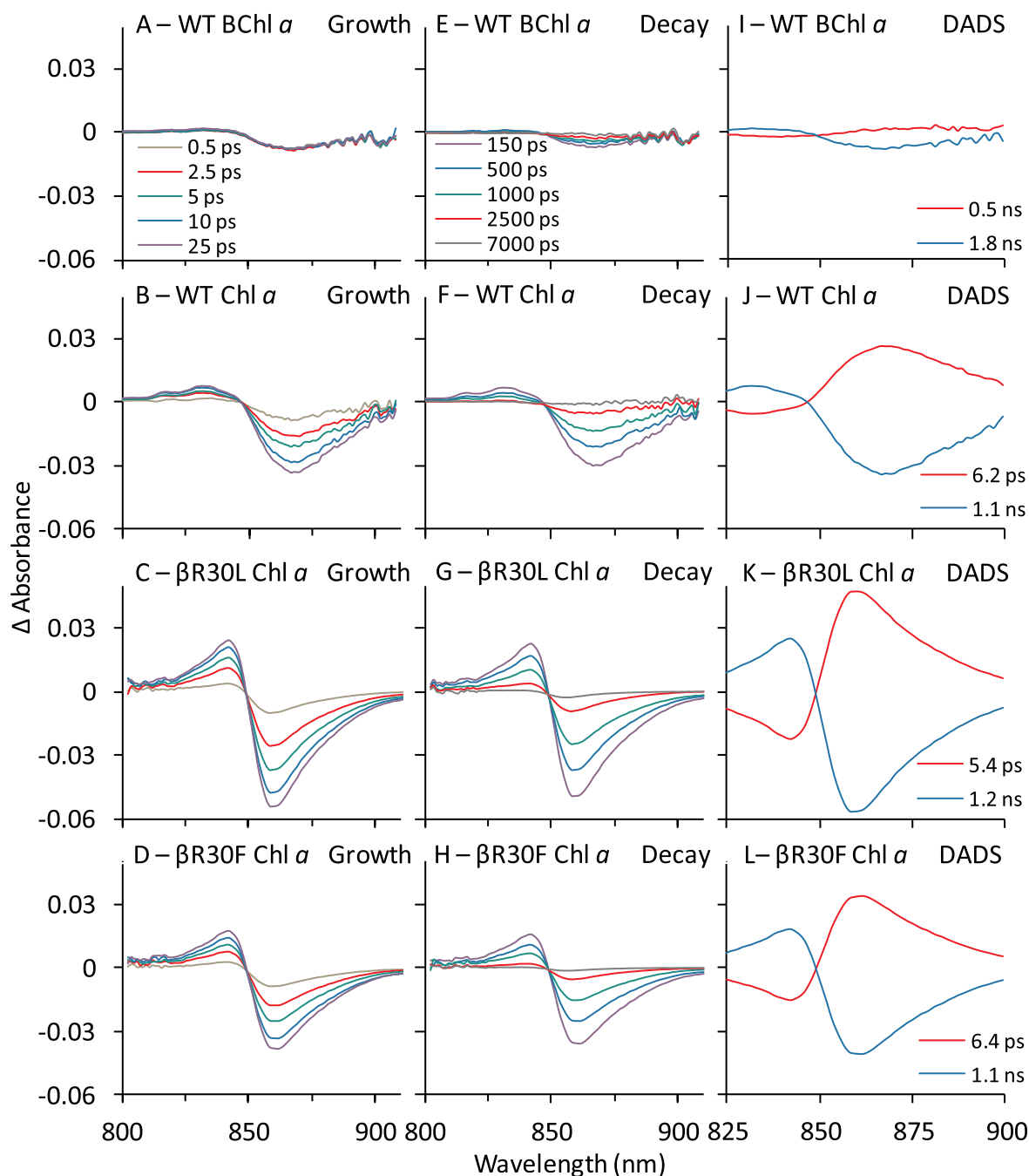
Fig. 6. A–H: NIR TA spectra for select Chl a -containing samples (and related controls) obtained at indicated times (indicated in Panels A and E) after excitation with a 100 fs pulse at 665 nm. Spectra were normalised to absorbance of B850 band. Panels A–D show growth of B850* and panels E–H the decay of B800*. Panels I–L show DADS obtained from global analysis of the data sets. The DADS in red (6–10 ps) in J–L reflect decay of Chl a * (primarily energy transfer to B850) and the DADS in blue (~1 ns) in (I–K) is for decay of B850* to the ground state.
