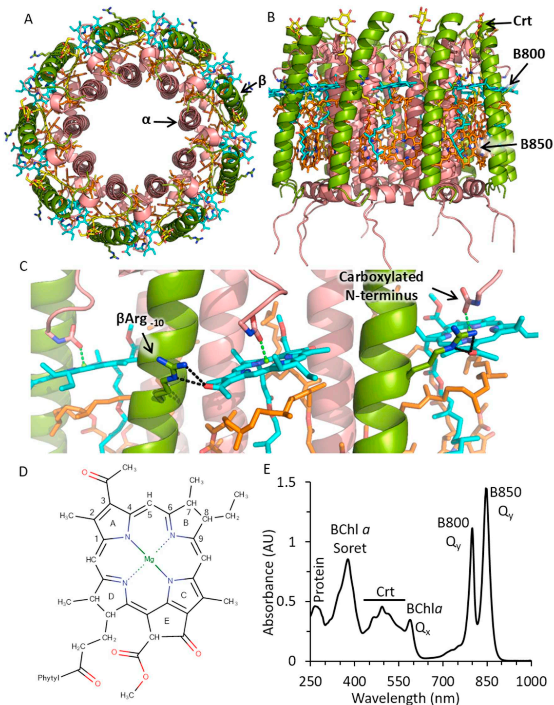
Fig. 1. Crystal structure of the Rba. acidophilus LH2 complex (PDB ID:1NKZ) [14]. The \alpha and \beta polypeptides are drawn as cartoons in pink and green, respectively. The \beta Arg -10 residue, the carboxylated N-terminus of the \alpha -subunit, and bound cofactors are drawn with sticks. B800 BChl a is cyan, B850 BChl a is orange and the carotenoid (Crt), rhodopin glucoside, is yellow. Annotated views from the top (panel A), side (panel B) and of the B800 site (Panel C) are shown. H-bonds to the \beta Arg -10 residue are shown with dashed black lines, and ligation of Mg by the carboxylated N-terminus is shown with green dashed lines. Panel D shows a 2D schematic of the BChl a structure annotated with ring lettering and numbering of porphyrin carbons 1–9. Panel E shows an annotated UV/Vis/NIR absorption spectrum of Rba. sphaeroides LH2.
