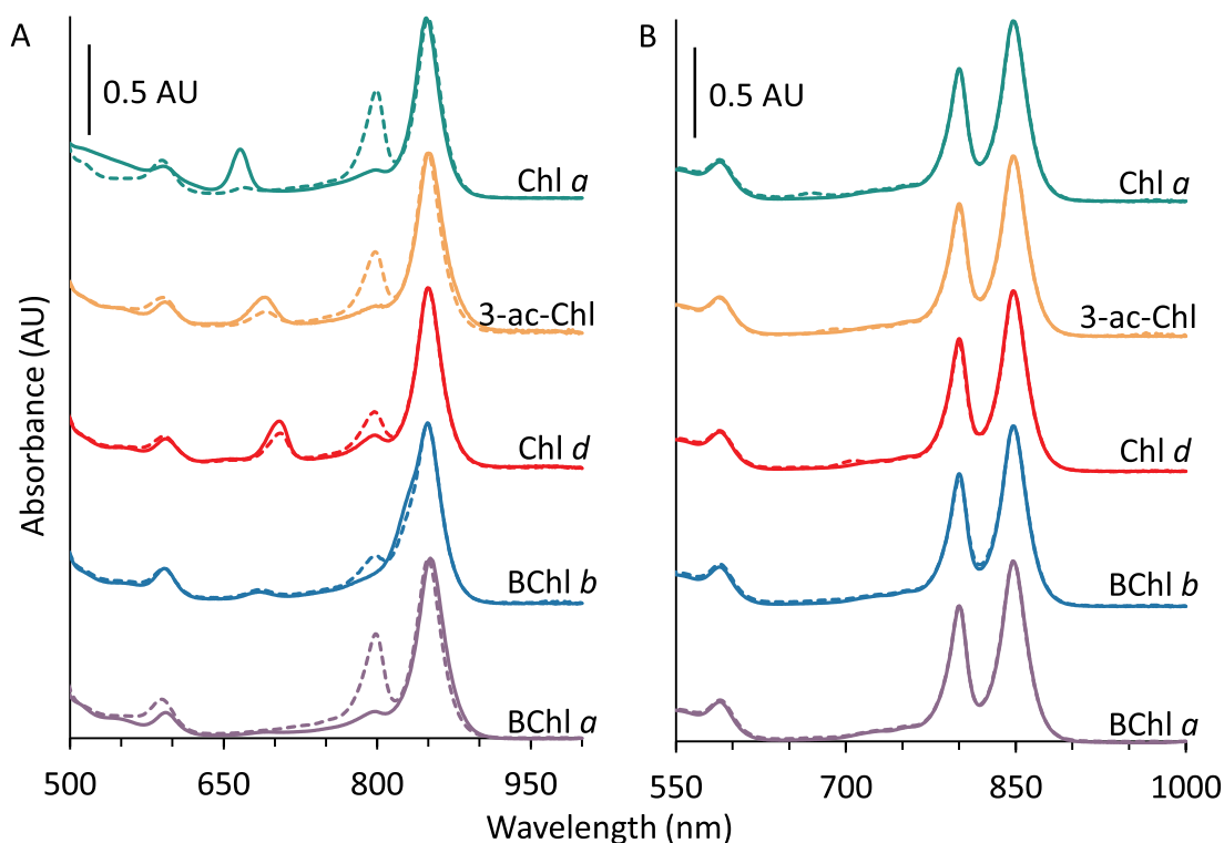
Fig. 3. Panel A: Solid lines show absorption spectra of WT B850 LH2 (Purple), and WT B850 reconstituted with Chl a (green), 3-acetyl-Chl a (orange), Chl d (red) or BChl b (blue). Dashed lines show the spectra of the B800-substituted complexes following incubation with excess BChl a and removal of free pigment. Panel B: WT (B800–850) LH2 before (solid lines) and after (dashed lines) incubation with Chl a (green), 3-acetyl Chl a (orange), Chl d (red), BChl b (blue) and BChl a (purple).
