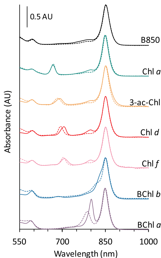
Fig. 5. Absorption spectra of WT (solid lines) and \beta R30L (dashed lines) B850 LH2 complexes (black), and B850 complexes reconstituted with Chl a (green), 3-acetyl-Chl a (orange), Chl d (red), Chl f (pink) and BChl b (blue). Purple lines show as-prepared BChl a containing complexes.
