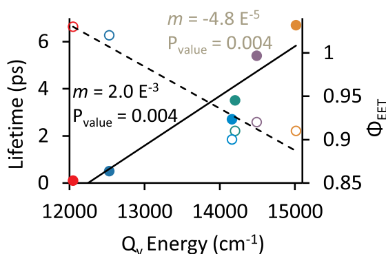
Fig. 9. Trends in (B)Chl lifetime (black line and filled symbols) and energy transfer efficiency ( \Phi_{\text{EET}} , dashed line and open symbols) as related to Q_y energy. The symbols representing the (B)Chls are as follows: BChl b -LH2 (red), BChl a -LH2 (WT, blue), Chl f -LH2 (cyan), Chl d -LH2 (green), 3-acetyl Chl a -LH2 (purple), and Chl a -LH2 (orange).
