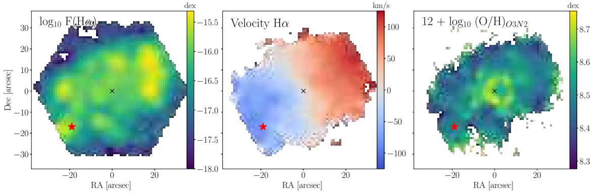
Figure A1. 2MASXJ07470232+2646347, the host of SN 2017ixz in H\alpha flux (left), H\alpha velocity (centre), and oxygen abundance (right).
