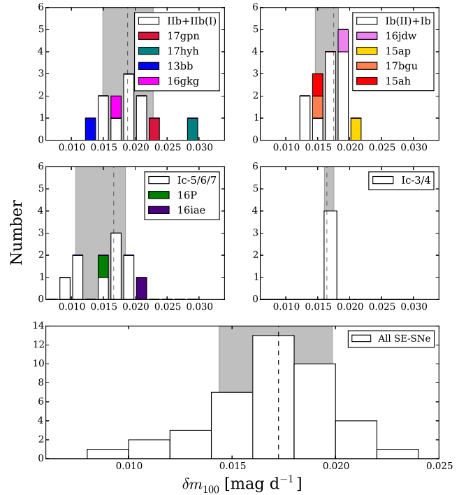
Figure 12. (top) The distribution of late time decay rates for SE-SNe; the median is \sim 0.017 mag \text{d}^{-1} for all SN types. Only SN 2013bb has had host-galaxy flux subtracted, but the effect of this on \delta m_{100} was found to be negligible at this phase, \sim 0.001 mag \text{d}^{-1} . The dashed line and grey regions are as in Figure 9.
