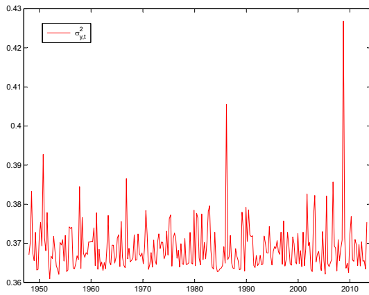
Figure 3: Time plot of the expected value of p(\sigma_{y,t}^2|y_1, \dots, y_T) , t = 1, \dots, 261 , obtained from the AR-S-TVP-SVC model.
