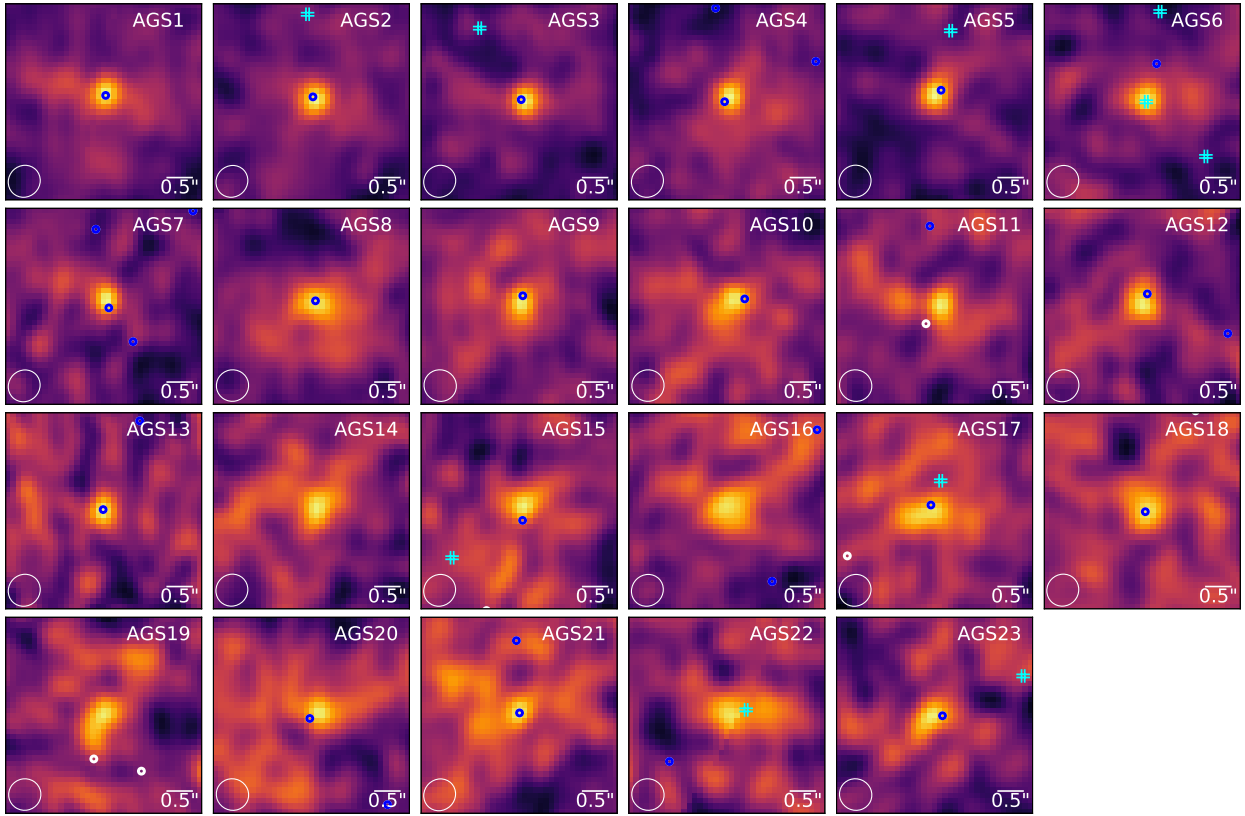
Fig. 8. ALMA 1.1 mm continuum maps for the 23 detections tapered at 0.60 arcsec. Each 3''.5 \times 3''.5 image is centered on the position of the ALMA detection. Cyan double crosses show sources from the GOODS- S CANDELS catalog. White circles show sources from the ZFOURGE catalog. Blue circles show common sources from both optical catalogs (sources with an angular separation lower than 0''.4 ). The shape of the synthesized beam is given in the bottom left corner.
