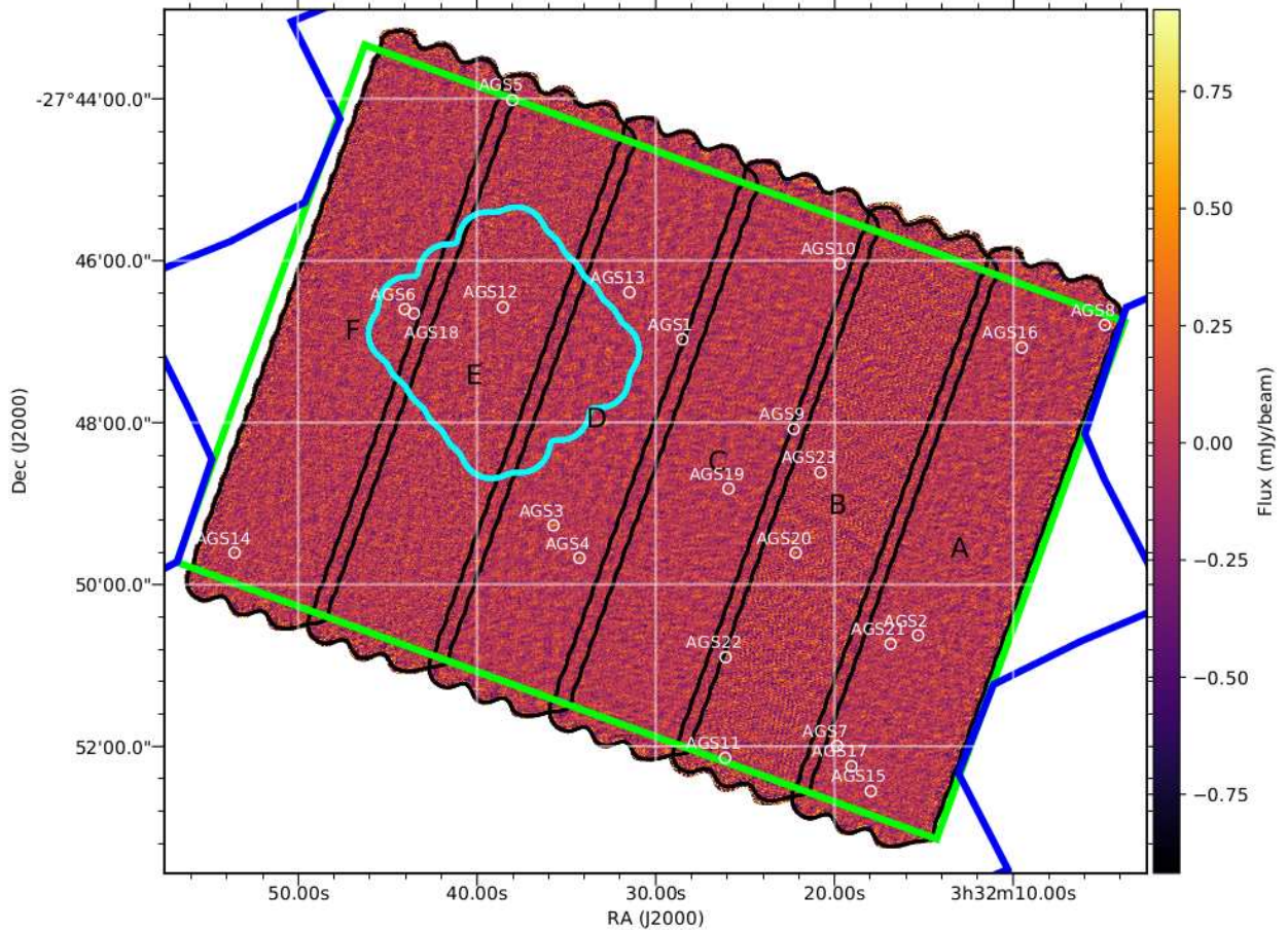
Fig. 1. ALMA 1.1 mm image tapered at 0''60 . The white circles have a diameter of 4 arcseconds and indicate the positions of the galaxies listed in Table 3. Black contours show the different slices (labeled A–F) used to compose the homogeneous 1.1 mm coverage, with a median rms-noise of 0.18 mJy per beam. Blue lines show the limits of the HST/ACS field and green lines indicate the HST-WFC3 deep region. The cyan contour represents the limit of the Dunlop et al. (2017) survey covering all the Hubble Ultra Deep Field region. All of the ALMA-survey field is encompassed by the Chandra deep field-South.
