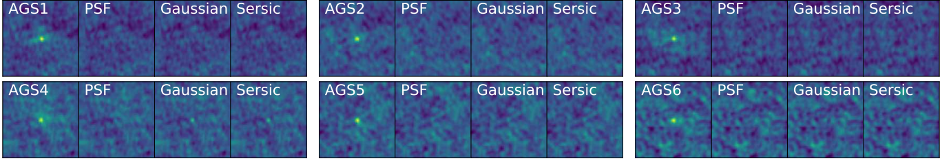
Fig. 11. 10'' \times 10'' postage stamps, centered on the galaxy detections. Left to right: source in the 0.6'' -mosaic map, and residuals obtained after PSF, Gaussian and Sersic flux fitting. The residuals are very similar between the three different extraction methods. Only the 6 brightest galaxies are shown.
