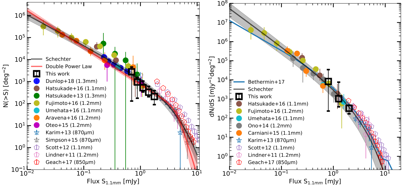
Fig. 16. 1.1-mm cumulative ( left panel ) and differential ( right panel ) number counts derived using the corrections described in Sect. 5.4, for the sources detected at >4.8\sigma in the main catalog. AGS19 is located at a position where the noise is artificially low, and has therefore not been taken into account. Previous (sub)millimeter cumulative number counts are also shown (Lindner et al. 2011; Scott et al. 2012; Karim et al. 2013; Hatsukade et al. 2013, 2016; Ono et al. 2014; Simpson et al. 2015b; Oteo et al. 2016; Carniani et al. 2015; Aravena et al. 2016; Fujimoto et al. 2016; Umehata et al. 2017; Geach et al. 2017; Dunlop et al. 2017). The different fluxes are scaled to 1.1 mm flux densities using S_{1.1\text{mm}}/S_{1.2\text{mm}} = 1.29 , S_{1.1\text{mm}}/S_{1.3\text{mm}} = 1.48 , S_{1.1\text{mm}}/S_{870\mu\text{m}} = 0.56 . From the Umehata et al. (2017) study, we used only sources which do not have z = 3.09 , (which means we are excluding the protocluster members). Results from single-dish surveys are shown with unfilled pentagon markers and are only indicative, they are not considered for model fitting. The gray curve shows the best-fit Schechter function (with 1-\sigma uncertainties), the red curve shows the best-fit DPL function (with 1-\sigma ).
