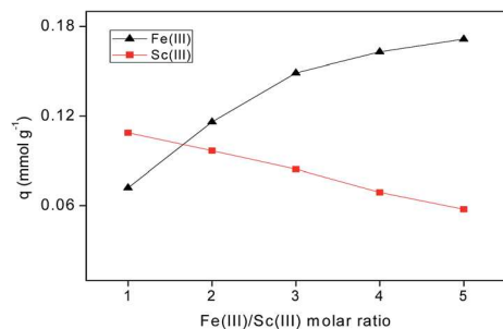
Fig. 11 Fe(III)/Sc(III) selectivity for the SILP Hbet-STFSI-PS-DVB: aqueous phase = 10 mL, 0.05 g of SILP, c_{in}[\text{Sc(III)}] = 1.1 \text{ mmol L}^{-1} , c_{in}[\text{Fe(III)}] from 1.1 \text{ mmol L}^{-1} to 5.5 \text{ mmol L}^{-1} , pH_{in} \approx pH_{eq} \approx 1.0 , 90 min, 300 rpm, room temperature.
