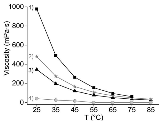
Fig. 5 Viscosity as a function of the temperature and the organic phase composition: (1) pure Cy923, (2) 20 v% Cy923 in [C101][NO 3 ], (3) 10 wt% Cy923 in [C101][NO 3 ] and (4) pure [C101][NO 3 ] and (4) after loading 39 g L -1 of REE in 20 v% Cy923 in [C101][NO 3 ].
