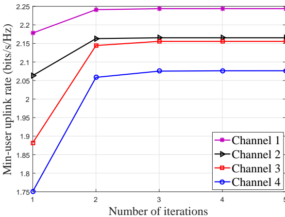
Figure 9. The convergence of the proposed max-min SINR approach (Algorithm 1) for M = 150 , K = 50 , D = 1 \text{ km} , and the length of the pilot sequences is set to 30 ( \tau = 30 ).
