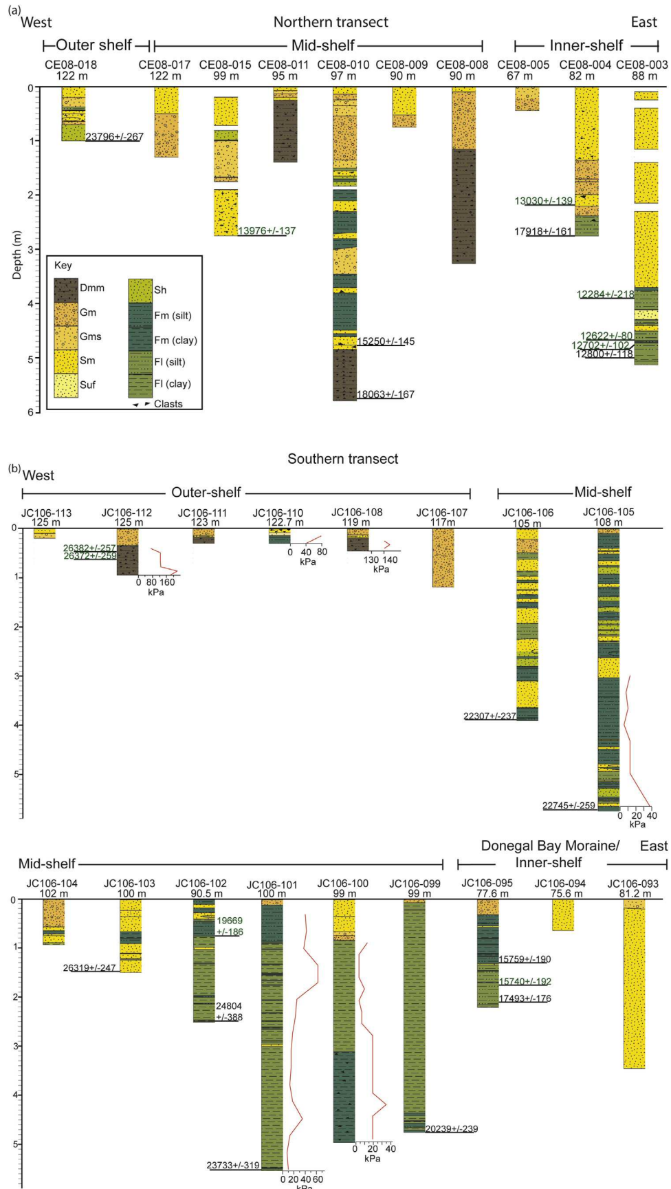
Fig. 6. Core logs presented as a west to east transect from outer shelf to inner shelf. The lithofacies are colour coded. Radiocarbon dates are shown alongside the logs at their stratigraphic depth. Dates in green are from shells, dates in black are from benthic foraminifera. (a) Northern core transect (Celtic Explorer cruise CE08 cores; see Fig. 1). (b) Southern core transect (James Cook cruise JC106 cores; see Fig. 1). Shear strength profiles (in kPa) are also shown in b. (For interpretation of the references to colour in this figure legend, the reader is referred to the Web version of this article.)
