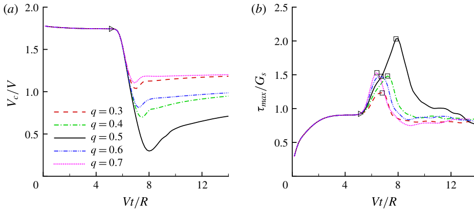
FIGURE 8. (Colour online) Capsule in the branched tube at different branch flow ratios ( a/R=0.4 , Re=0.25 , Ca=0.5 ). Time evolution of (a) the velocity magnitude V_c/V , and of (b) the maximum principal tension. The squares indicate the dimensionless times when \tau_{max} reaches its peak value. The corresponding positions of the capsule centre of mass are shown in figure 6. The triangle denotes the position where the bifurcation starts to affect the capsule motion.
