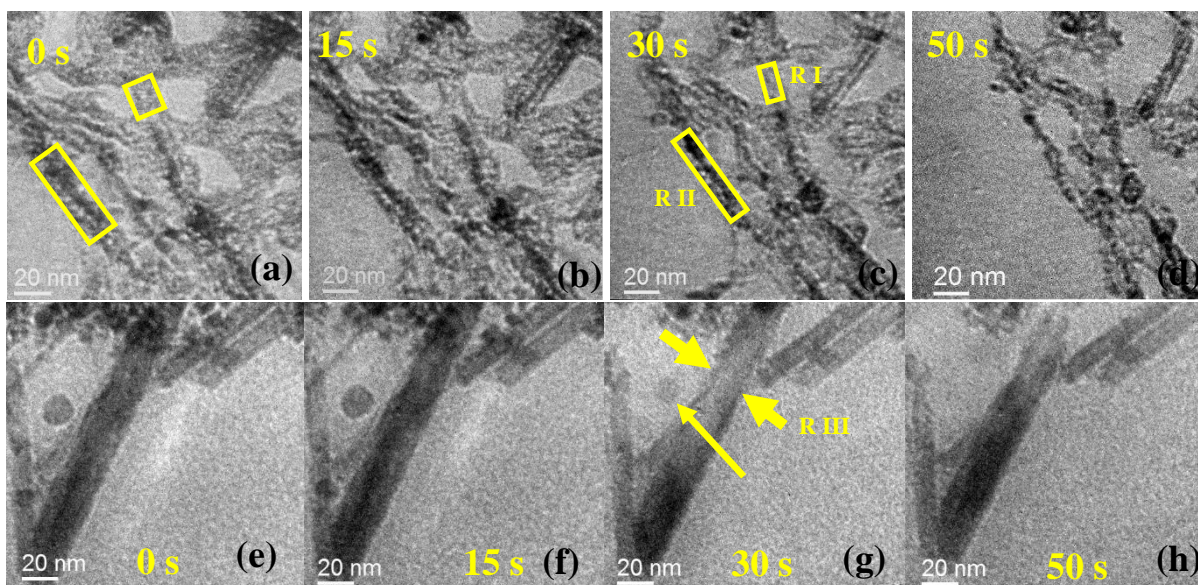
FIG 3: Dissolution of ceria nanorods (a-d) involving rough surface (JEM 2010-F at 200kV; boxes indicate measured items for table 1). (e-h) dissolution of straight, smooth and homogeneous ceria nanorod along with one round nanoparticle (JEM-2010-F at 200kV; arrows indicate measured items for table 1).
