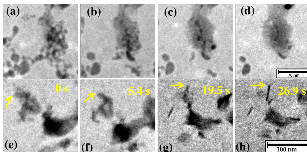
FIG. 4 Parallel formation and dissolution: (a-d) Growth of amorphous phase around and replacing raw nanoparticles. (e-h) Transformation of 3D irregular shaped particles into needle shaped particles. The arrow helps tracking one corner of a particle rotating while transforming.
