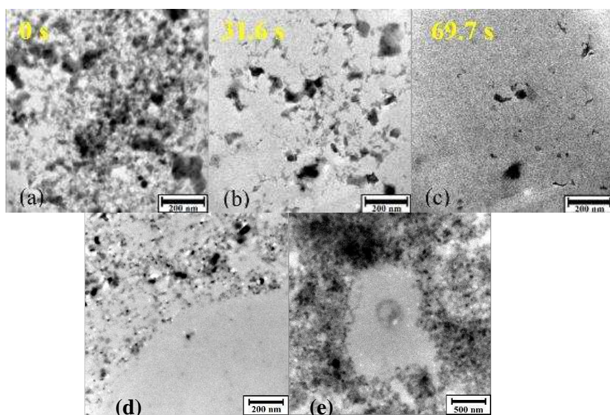
FIG. 1 (a-c) Aqueous dissolution of ceria nanoparticle powder during electron irradiation; (d, e) Comparison of sample before and after irradiation-dissolution: beam shift (d) and magnification-reduction (e) illustrating sharp circular borderline between the regions inside (no particles) and outside (original particles) the irradiation zone.
