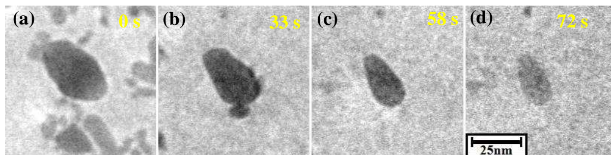
FIG. 2 Sequence of ceria dissolution: (a-d) ceria nanoparticle involving particle aspect ratio increase before complete dissolution; (JEM 3010 at 300kV).
