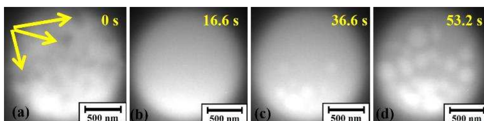
FIG. 6 Nano bubble formation and their growth at very high intensity of electron beam irradiation with (a) yellow arrows showing residual nanoparticles, (b) complete dissolution of CNPs, (c) bubble formation and (d) growth of bubbles.
