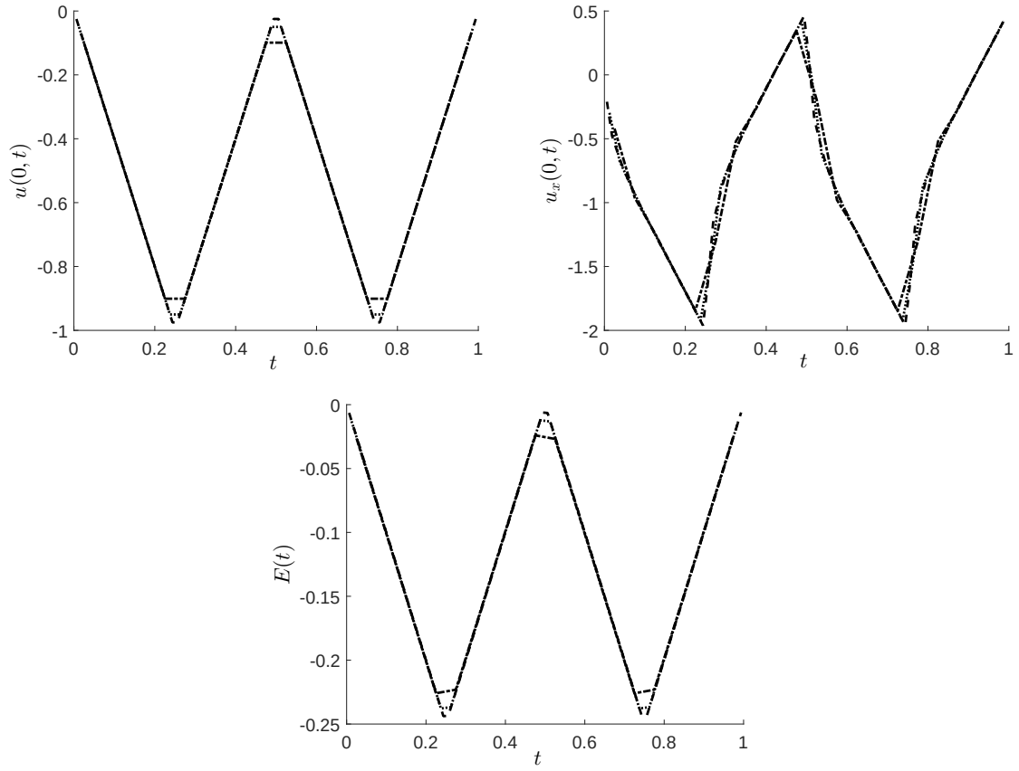
Figure 4: The numerical results of u(0,t) , u_x(0,t) and E(t) obtained by solving the direct problem (2.2)–(2.4), (2.15) using the BEM with N = N_0 = \{20(-\cdot-), 40(\cdots), 80(-\cdot-\cdot-)\} , for Example 2.
