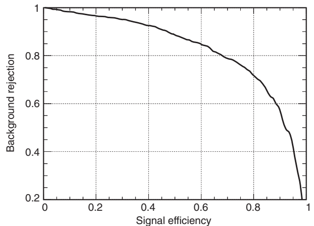
FIG. 10. Efficiencies of signal selection and background rejection by cutting the NN output in SK-IV.
