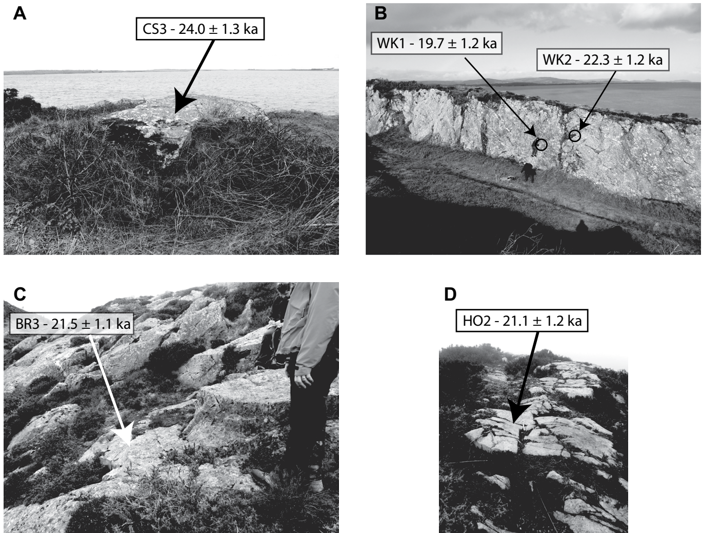
Figure 5. Photographs of selected cosmogenic nuclide (CN) samples discussed in the text. (A) Boulder incorporated at Carnsore point, Co. Wexford, Ireland. (B) Wicklow meltwater channel showing the location of samples collected. (C) Plucked lee slope on Bray Head, Co. Wicklow, Ireland, sampled for CN dating (ice flow right to left). (D) Glacially abraded surface on summit of Hill of Howth, Co. Dublin, Ireland. Striations and small scale p-forms are preserved (ice flow toward camera). Location of sample HH2 is shown. HH1 was collected from a similar outcrop of abraded quartzite bedrock.
