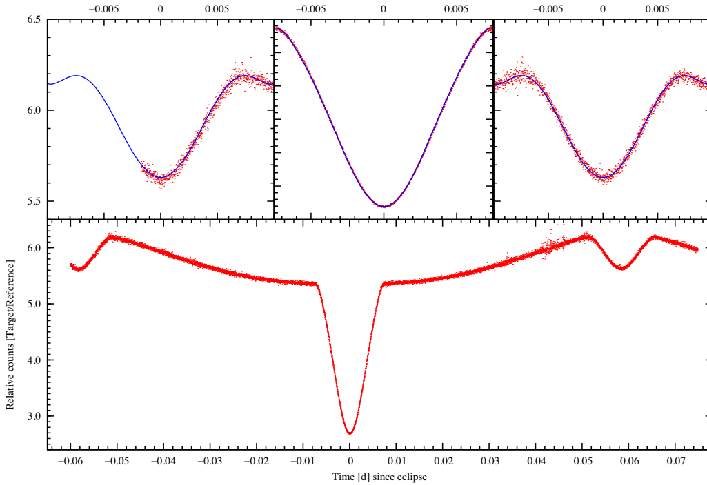
Figure 9. Ultracam light curve. The data shows observations in the g -band and fits to the primary and two secondary eclipses.
