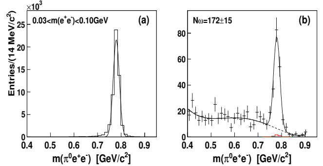
FIG. 12: (Color online) Same as Fig. 11, but after applying the softer cuts on N and R (depicted by red dashed lines in Fig. 3) and the dE/dx cut rejecting events with twice the magnitude of a signal from a single e^{+/-} in one PID element.
