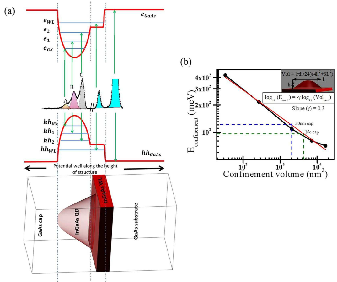
Figure 5. (a) Correlation between structure of QDs and obtained PL lines are linked by the excitonic level formation inside the QDs and WLs. Different PL lines (for 5 nm GaAs cap sample) has been associated with the composition and shape dependent exciton levels of QDs. (b) The variation of confinement energy with respect to the confined volume for lens shape InGaAs quantum dots. Black dots are the obtained values of electron ground state energy and heavy hole ground state energy 34 . Red line is the least square fitting of the data points which shows slope of 0.3. Blue line and green line indicate the confinement energy values for confinement volume 2049 nm 3 and 4080 nm 3 of lens shaped QDs for 30 nm capped and uncapped sample in GID respectively.
