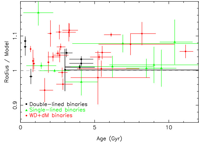
Figure 8. The over-inflation of M dwarfs as a function of their ages. Measured radii were compared to the closest Baraffe et al. (2015) model in age.
