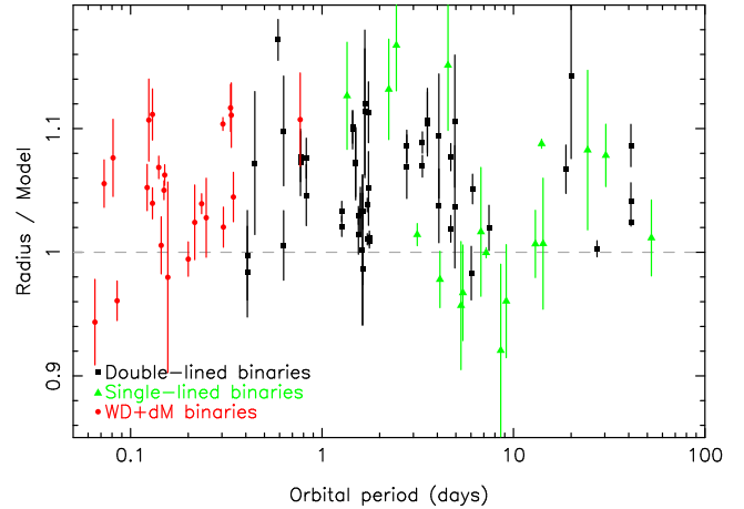
Figure 10. The over-inflation of M dwarfs as a function of their orbital period. Note that many stars in systems with periods longer than a few days are not synchronously rotating (usually rotating slower than the binary period) and generally have moderately eccentric orbits.
