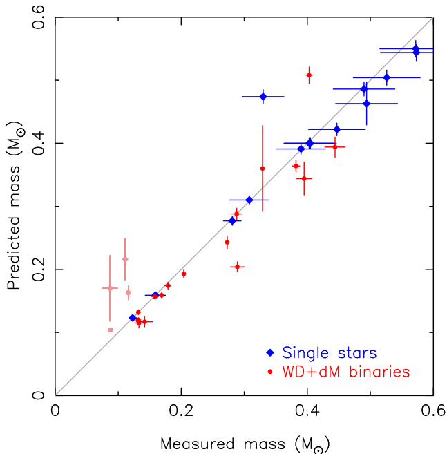
Figure 7. The measured masses of M dwarfs compared to those derived using the empirical mass- M_{K_s} relation from Mann et al. (2018). Faded red points are binaries where the white dwarf still contributes a substantial amount of the flux in the K_s band and therefore may not have reliable predicted masses.
