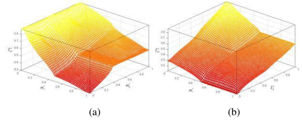
Figure 5. Fuzzy surface of the evaporator outlet temperature with respect to \bar{m}_r and \bar{m}_h (a), and with respect to \bar{m}_r and T_h (b)
