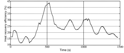
Figure 16. Heat recovery efficiency
