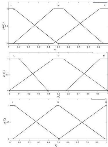
Figure 3. Membership functions of input variables.
