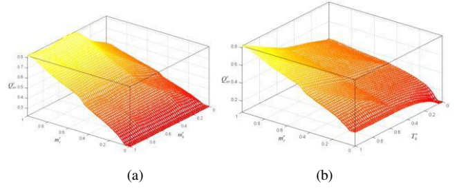
Figure 6. Fuzzy surface for the evaporator power with respect to \bar{m}_r and \bar{m}_h (a), and with respect to \bar{m}_r and T_h (b)
