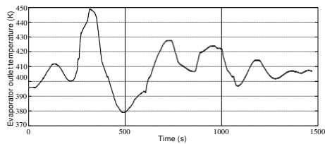
Figure 13. Evaporator outlet temperature
