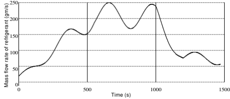
Figure 11. Mass flow rate of refrigerant
