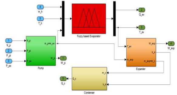
Figure 10. Overall model of the ORC-WHR system.
