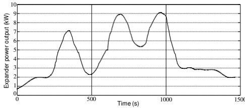
Figure 14. Expander power output.
