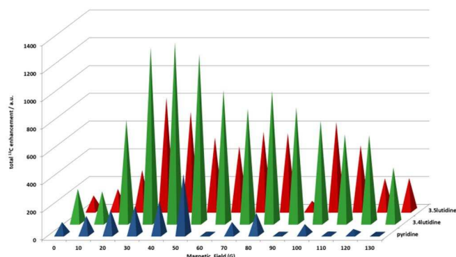
Fig. 6. Graph comparing the ^{13}\text{C} enhancement observed for the carbon resonances of pyridine, 3,4-lutidine and 3,5-lutidine when using complex 3d as a function of the strength of the polarisation transfer field.
