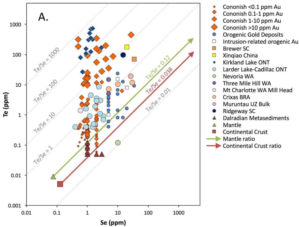
Fig. 1. Whole rock geochemistry A) Te-Se data and B) Te-Au data, for the Cononish deposit, Scotland, compared with other gold deposits in orogenic belts (circles), bulk continental crust and mantle, and local Dalradian metasediment host-rocks. Where specified, intrusion-related orogenic gold deposits are plotted separately with square symbols, although appear to follow the same trends. Some notable deposits are specifically named. Cononish and Dalradian metasediment data were analysed by OMAC for Scotgold using fire assay-AA for Au and four acid digest and ICP-OES/AES/MS procedures for Te and Se (Hill, 2014). Most other data are from the OSNACA dataset (Brauhart et al., 2017), except: Kirkland Lake, Larder Lake-Cadillac data (Ispolatov et al., 2008); Muruntau (Koneev et al., 2005); Mt Charlotte (Mueller, 2015); continental crust (Wedepohl, 1995; Rudnick and Gao, 2014); mantle (Palme and O’Neil, 2014).
