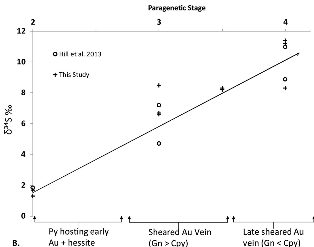
Fig. 7. A. Histogram of compiled pyrite \delta^{34}\text{S} for the Cononish deposit. B. Pyrite \delta^{34}\text{S} vs. paragenetic stage.
