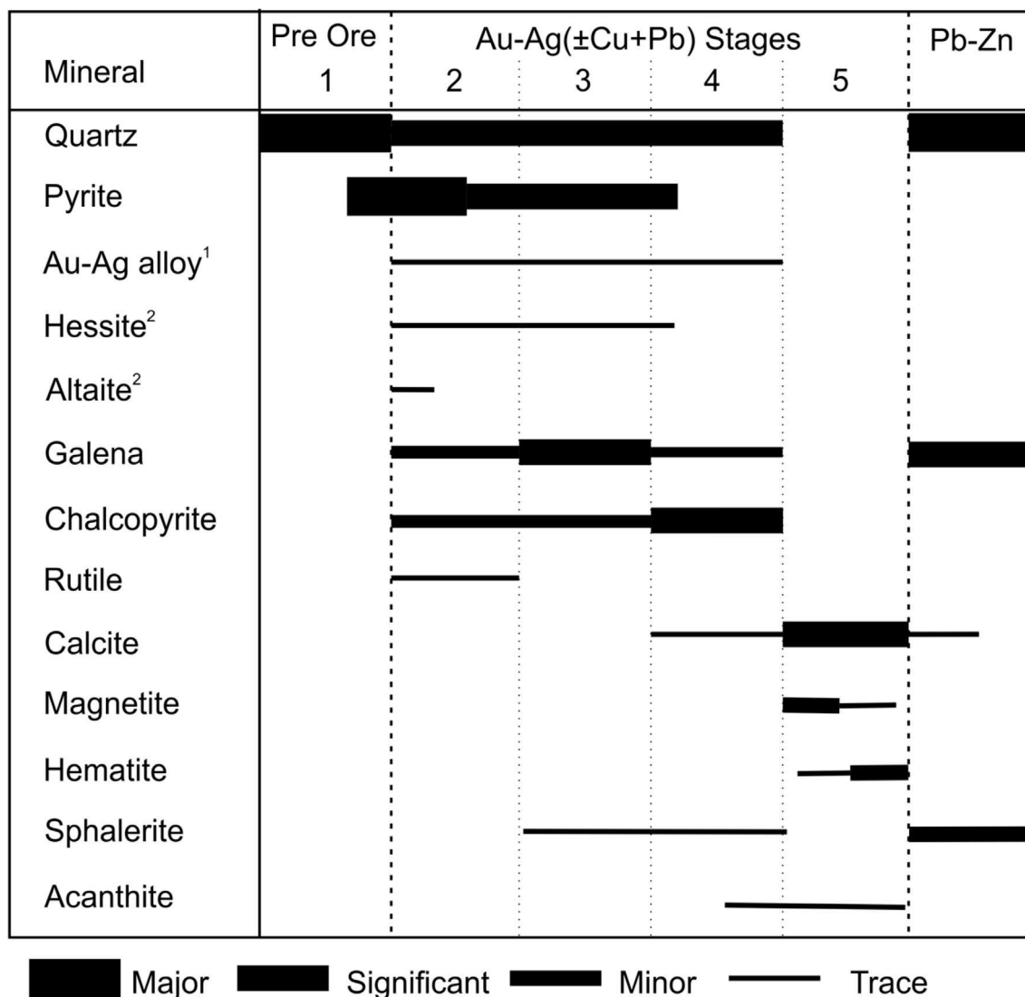
Fig. 4. Paragenesis for the Cononish Au-Ag ( \pm Cu, Pb) vein and later cross-cutting Pb-Zn vein. Estimated relative mineral proportions are shown by width of the bar. 1 Au content of the alloy is observed to decrease over time. 2 Abundance of tellurides decreases from stage 2 with very few tellurides observed in stage 3 mineralisation.
