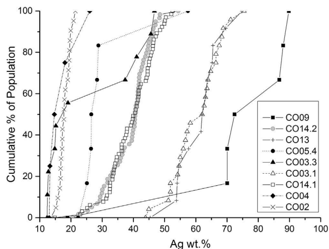
Fig. 5. Cumulative plot of the Ag wt% proportion of Au-Ag alloy grains measured in this study (n = 215) shown as populations of grains within an individual thin section. Each sample recorded a distinct and variable distribution of grain compositions dependent on the stages of the paragenetic sequence sampled. A limited number of the thin sections, such as CO03.3, CO04 and CO09, show a bimodal distribution of Au-Ag alloy composition that can be correlated with the observation that they contained two or more distinct gold bearing stages of the paragenesis.
