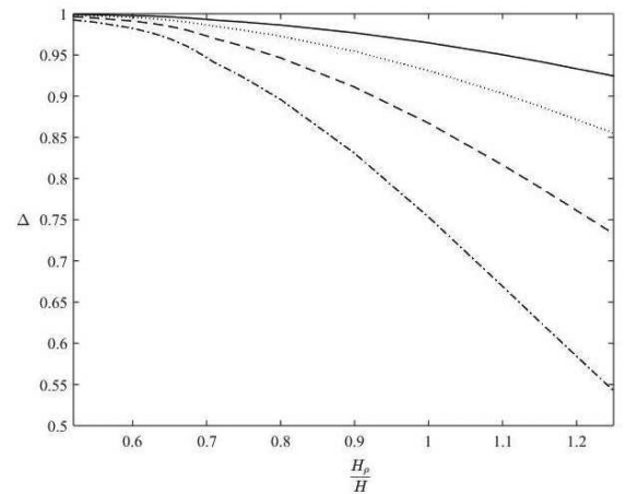
Figure 6. Dependence of \Delta calculated at z = 6H on H_\rho/H . This dependence is calculated for \nu = 10^7 \text{ m}^2 \text{ s}^{-1} . The solid curve corresponds to H = 30 Mm and the wave period 60 s, the dotted curve to H = 60 Mm and the wave period 60 s, the dashed curve to H = 30 Mm and the wave period 30 s, and the dash-dotted curve to H = 60 Mm and the wave period 30 s.
