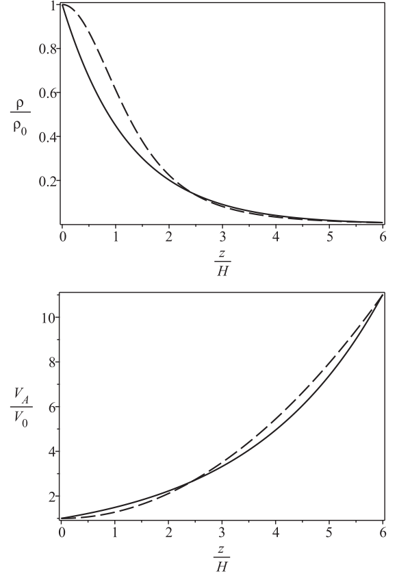
Figure A1. Dependence of \rho (upper panel) and V_A (lower panel) on z at r = 0 with the density defined by equation (104) (solid line) and by equation (A7) (dashed line) for H_\rho/H = 1.25 .
