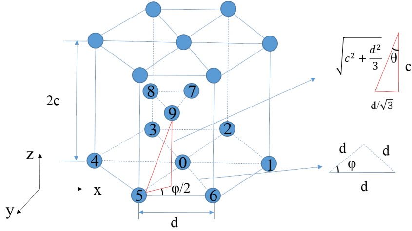
Figure 8: 3D HCP packing of DEM particles
