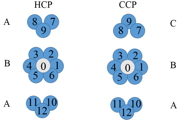
Figure 7: (a) HCP packing and (b) CCP packing [50]
