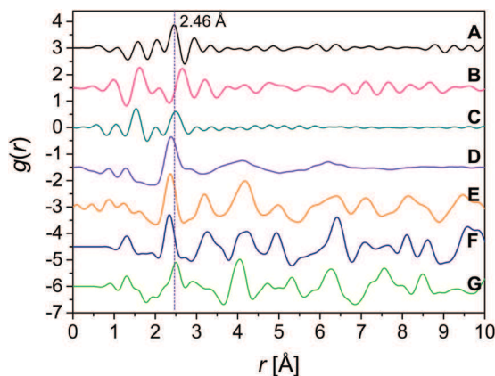
Fig. 4 Atomic PDFs of the aggregated globular \text{CaCO}_3 microemulsion compared to microemulsion components and standard solid \text{CaCO}_3 polymorphs. (A) A centrifuged 0.075 \text{ mol L}^{-1} \text{CaCO}_3 microemulsion at w = 10 (with isooctane background subtracted); the g(r) shows a characteristic unique peak at 2.46 \text{ \AA} and no structural coherence above \sim 4 \text{ \AA} . The peak can be attributed to a Ca–O distance; 43 (B) surfactant component of the microemulsion: 0.1 \text{ mol L}^{-1} NaAOT solution in isooctane with the medium subtracted as a background; (C) oil component of the microemulsion – pure isooctane; (D) solid amorphous calcium carbonate (ACC); (E) crystalline vaterite; (F) crystalline calcite; (G) crystalline aragonite; PDFs D–G were measured using dry powder samples. A characteristic “rippling” in patterns A to C at r > 4 \text{ \AA} is an artifact of the Fourier transform of the as-collected HEXD data and is a consequence of decreased signal-to-noise ratios in liquid samples compared to dry powdered samples shown in D–G.
