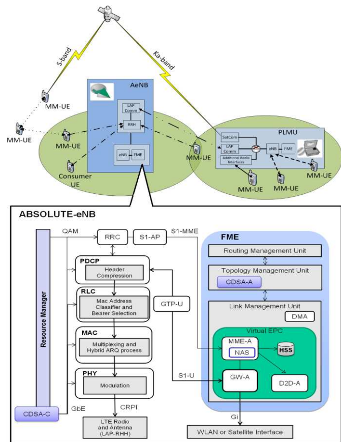
Figure 2. Units and agents of the flexible management entity.
