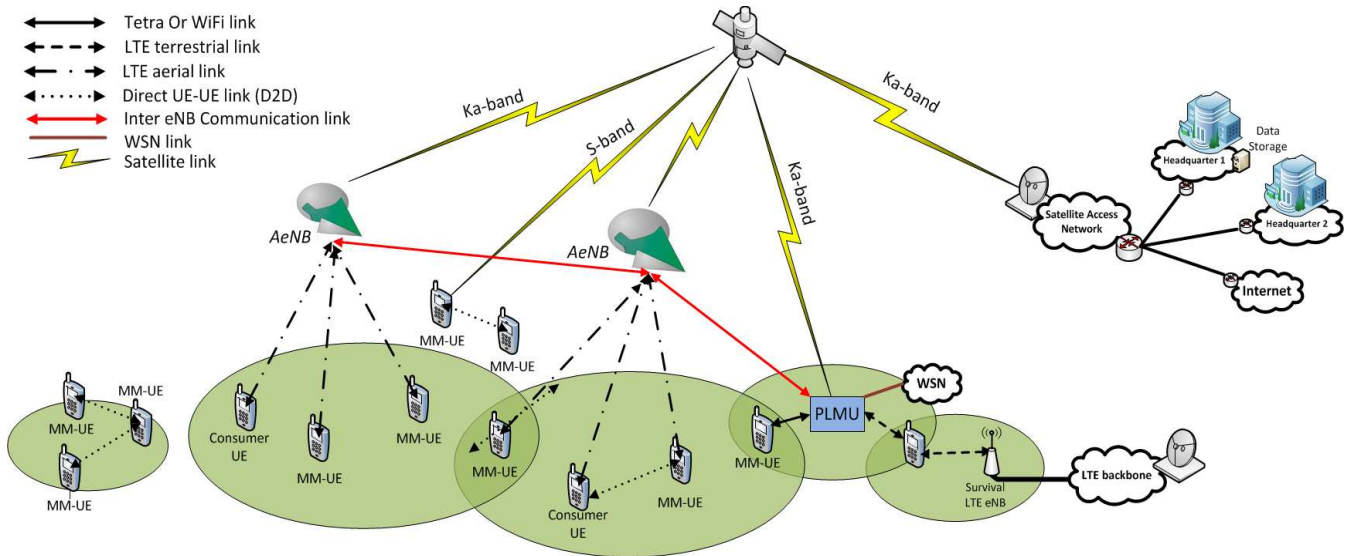
Figure 1. Overall ABSOLUTE architecture suitable for public safety scenarios. The main components of ABSOLUTE network are Aerial Base Stations (AeNBs), Portable Land Mobile Units (PLMUs), Ka-band Satellite Backhauling, S-MIM Satellite Messaging and Multimode User Equipment (which are able to operate in Direct Mode).
