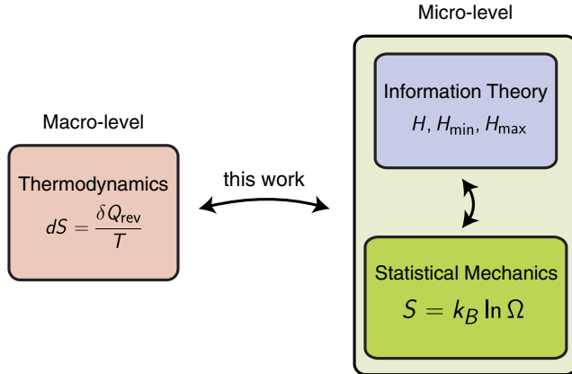
FIG. 1. The contribution of this Letter is to draw a connection between thermodynamic and information-theoretic entropy based on formal axioms and general principles such as additivity and monotonicity that are satisfied within both theories (Proposition 1). This replaces the textbook identification of entropy in thermodynamics and statistical mechanics based merely on analogies, such as common behavior of the two entropy functions in specific models like the ideal gas. The entropy functions in information theory and statistical mechanics are already formally equivalent, and conceptual links have been established through Jaynes’ maximum entropy principle [22], as well as through the works of Landauer [5] and Bennett [6] (based on explicit protocols that convert one into the other in an underlying microscopic model).
