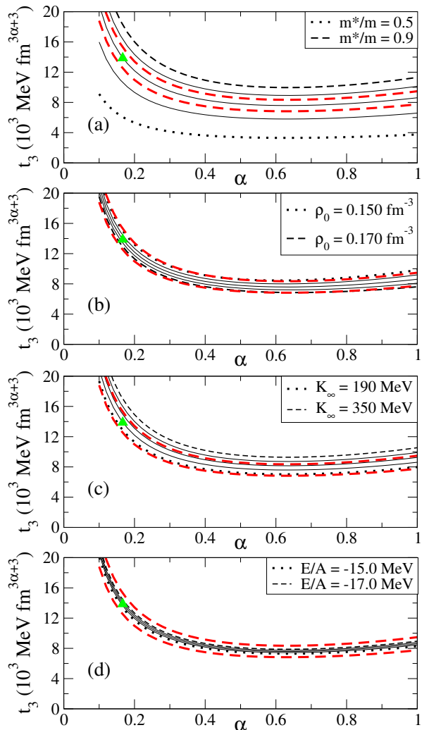
FIG. 1: (Color online) The parameter t_3 plotted as a function of \alpha for various sets of isoscalar bulk properties. In each case, one of the four bulk properties K_\infty , m^*/m , E/A , \rho_{\text{sat}} is varied keeping constant the three others (see text). The green triangle marks the SLy5* parametrization [15].
