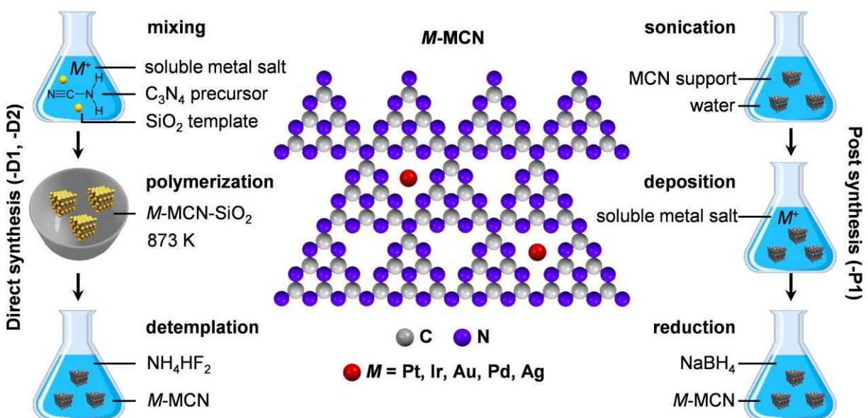
Figure 1. Direct synthesis (-D1, -D2) and post-synthesis (-P1) approaches to stabilize metal atoms within g- \text{C}_3\text{N}_4 , exemplified for the mesoporous MCN carrier. In the idealized location depicted, the metal atom is coordinated by up to 6 nitrogen atoms within interstices defined by the packing of the tri-s-triazine units.
