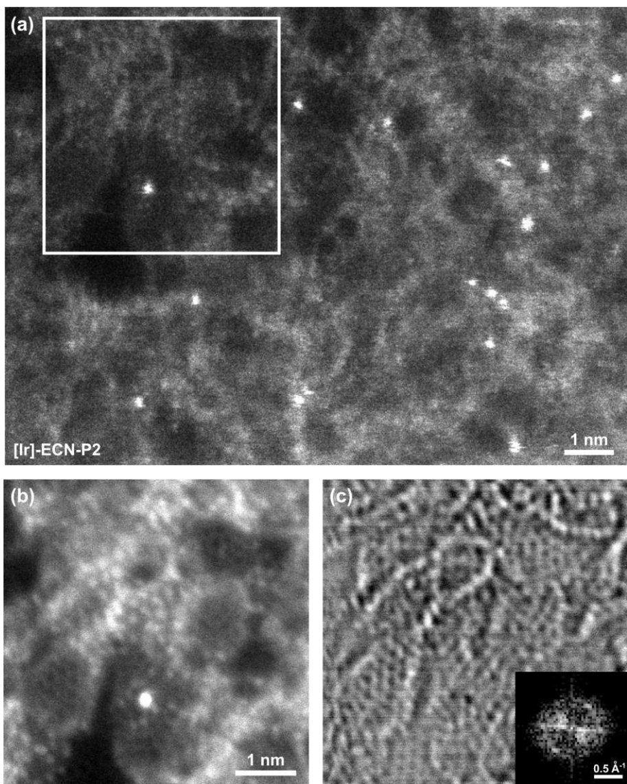
Figure 4. ‘Gentle STEM’ analysis of a model Ir SAHC. a) Attomically resolved STEM HAADF image showing Ir atoms distributed across the ECN support, b) simultaneous STEM HAADF and c) BF images of the boxed region in a). The inset in c) is a local Fourier transform taken from the lower left hand region of the image. These images are a sum of 50 frames acquired rapidly over approximately 50 s and summed to produce images with high contrast and clarity. The very bright dot in b) is a single Ir atom anchored on a g-C 3 N 4 raft.
