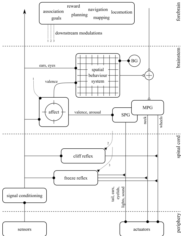
Figure 2: Illustration of MiRo 's control architecture loosely mapped onto brain regions (spinal cord, brainstem, forebrain). Signal pathways are excitatory (open triangles), inhibitory (closed triangles), or complex (closed circles). BG is the Basal Ganglia. SPG/MPG are the Social/Motor Pattern Generators.
