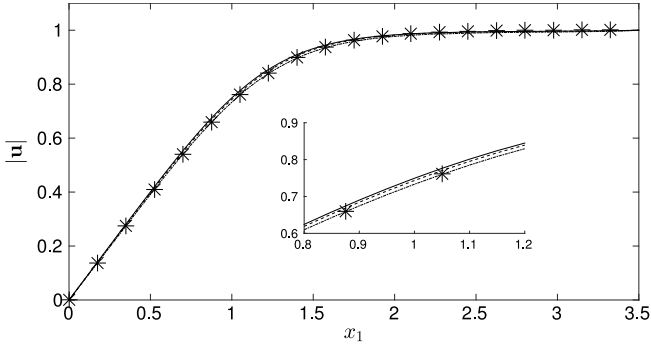
Fig. 6. The magnitude of the velocity along the center line. The numerical results for \mu_p = 0.5 and \delta = 0.1 for \lambda = 0, 0.1 and 0.2 are given by the solid, dashed and dot dashed lines respectively. The velocity given by the Padé approximation is given by asterisks.
