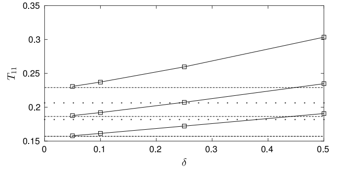
Fig. 9. T_{11} component of the extra stress at the stagnation point for W_e = 0 (bottom line), W_e = 0.1 , W_e = 0.2 (top line) with \mu_p = 0.1 for varying \delta . The Hele-Shaw ( \delta = 0 ) solutions are given by horizontal dashed lines for the weak-coupling solution and the dotted line for the second order fluid approximation respectively.
