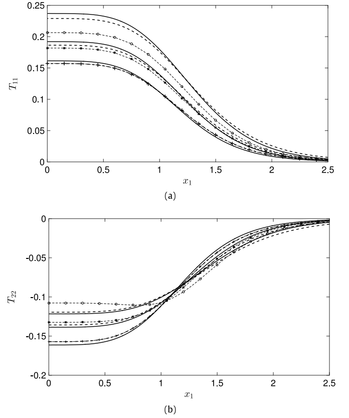
Fig. 7. Diagonal viscoelastic stress components with polymer viscosity \mu_p = 0.1 and \delta = 0.1 , (a) T_{11} , (b) T_{22} . The crossed, dotted and circular marked lines denote the SOF solution whereas the solid and dashed lines denote the FEM Oldroyd B model and similarly the weak coupling Padé solution respectively. The curves are given for W_e = 0, 0.1 and 0.2 , which go from bottom to top in (a), and top to bottom in (b).
