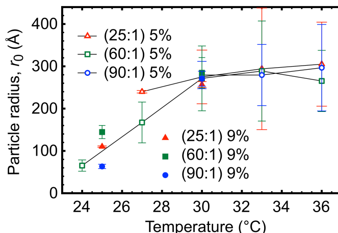
Figure 4. Temperature-dependent evolution of the particle radius, r_0 , obtained by fitting SANS data for 5 and 9 wt% HB-PNIPAMs in D 2 O above their LCST to scattering from disperse spheres. For the 5 wt% linear PNIPAM, the combined function (eqn 2) was used, and then only at 36°C to give r_0 = 0.127 \pm 0.004 \mu\text{m} (not shown)
