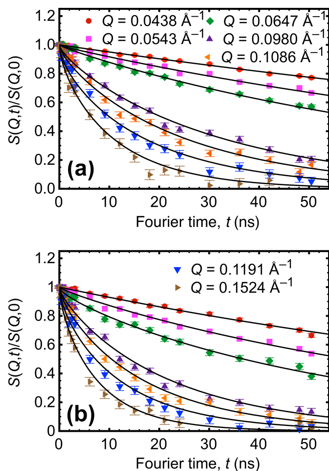
Figure 5. Intermediate scattering function for D7-HB-PNIPAM (a) (25:1) at 15.0 °C and (b) (90:1) at 24.0 °C in D 2 O at the values of Q indicated. The LCST of these polymers at the concentration of 4% (w/w) is 28°C and 30°C ( Table 3 ). The solid lines are fits to eqn 4 with \beta = 1/2
