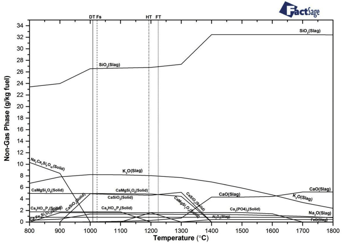
Fig. 7. Stable solid phases in equilibrium with the slag phase for 20% El Cerrajon coal 2 and 80% wheat straw co-combustion (BWCA82).
