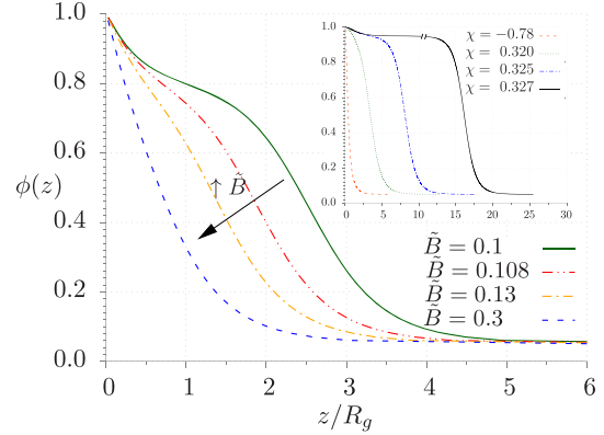
FIG. 3. Migrant concentration profiles \phi(z) for the SB model including the elasticity obtained by minimizing Eq. (4) for ( \chi = 0.320 and N_A = 10 ) and increasing \tilde{B} . A wetting transition is not observed in this model. Inset shows concentration profiles for the SB model without elasticity for the symmetric case N_A = N_B = 10 with increasing \chi . The black solid line with a break indicates the formation of a macroscopic wetting layer.
