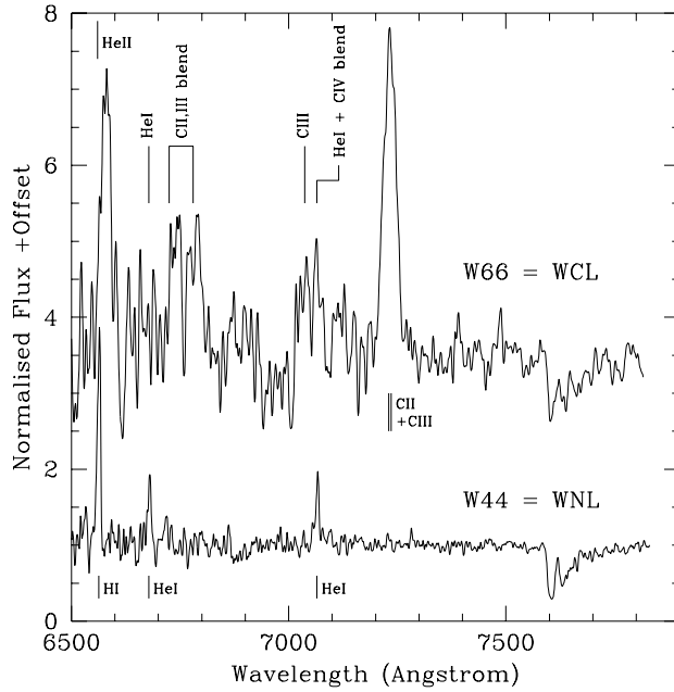
Fig. 2. R band spectra of the 2 newly discovered WR stars in the cluster; Candidate L (=W44), a probable WN9 star and Candidate M (=W66), a sixth WCL star (WC9).
