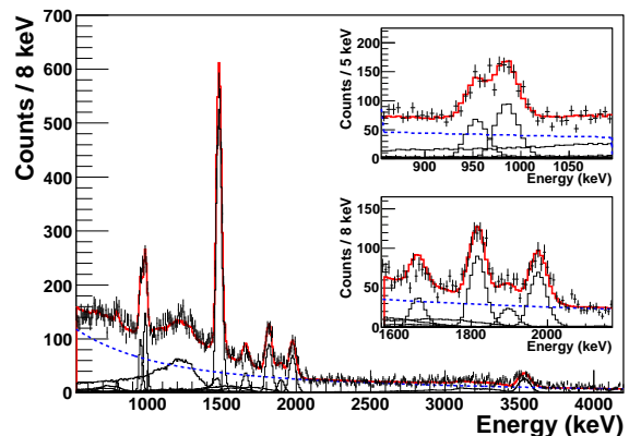
Figure 1: (Color online) Doppler corrected and add-back reconstructed \gamma -ray energy spectrum ( E_\gamma > 500 keV) in coincidence with ^{30}\text{Mg} . The overall fit (red line) includes Geant4 generated lineshapes for each transition (black histograms) and an exponential background (blue dashed line). The insets show the details of the regions from 850 to 1100 keV and 1575 to 2175 keV.
