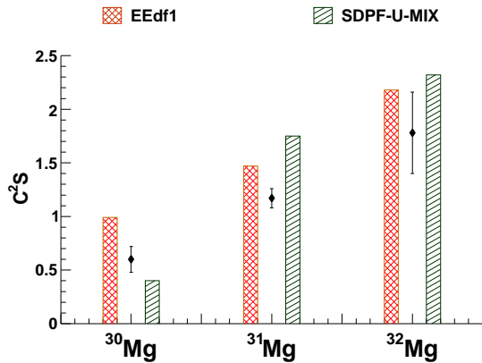
Figure 7: (Color online) Comparison of the experimentally deduced summed strength for neutron fp -shell levels populated in one-neutron removal from ^{30-32}\text{Mg} with shell-model predictions using the EEdf1 and the SDPF-U-MIX interactions. The experimental strengths (points with error bars) for ^{30,32}\text{Mg} are taken from Ref. [18].
