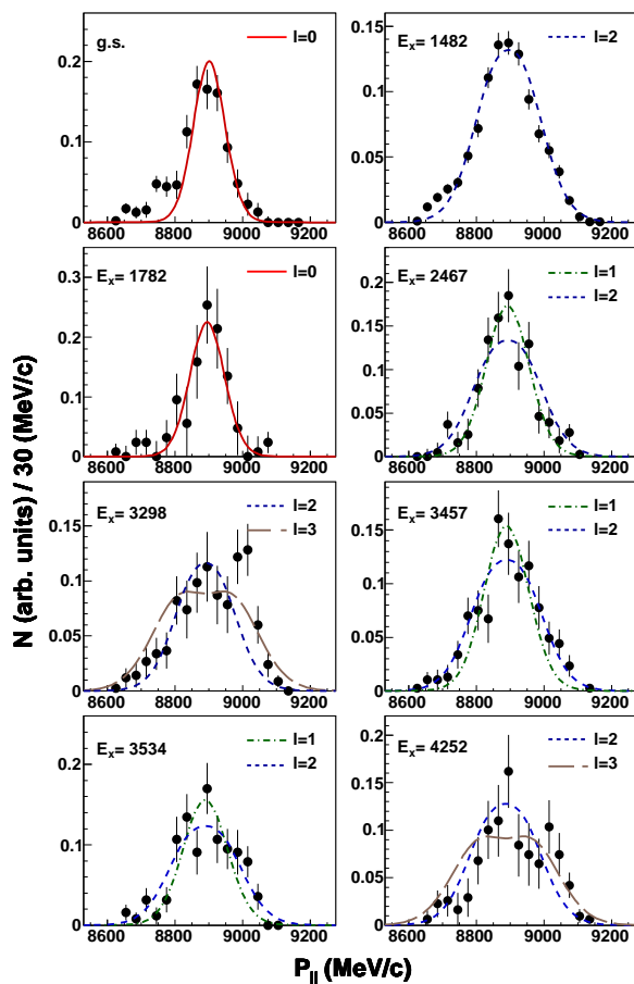
Figure 4: (Color online) Exclusive momentum distributions derived for states in ^{30}\text{Mg} , labelled by the excitation energy in keV, compared to eikonal-model predictions; fits were for momenta above 8750 MeV/c (see text).
