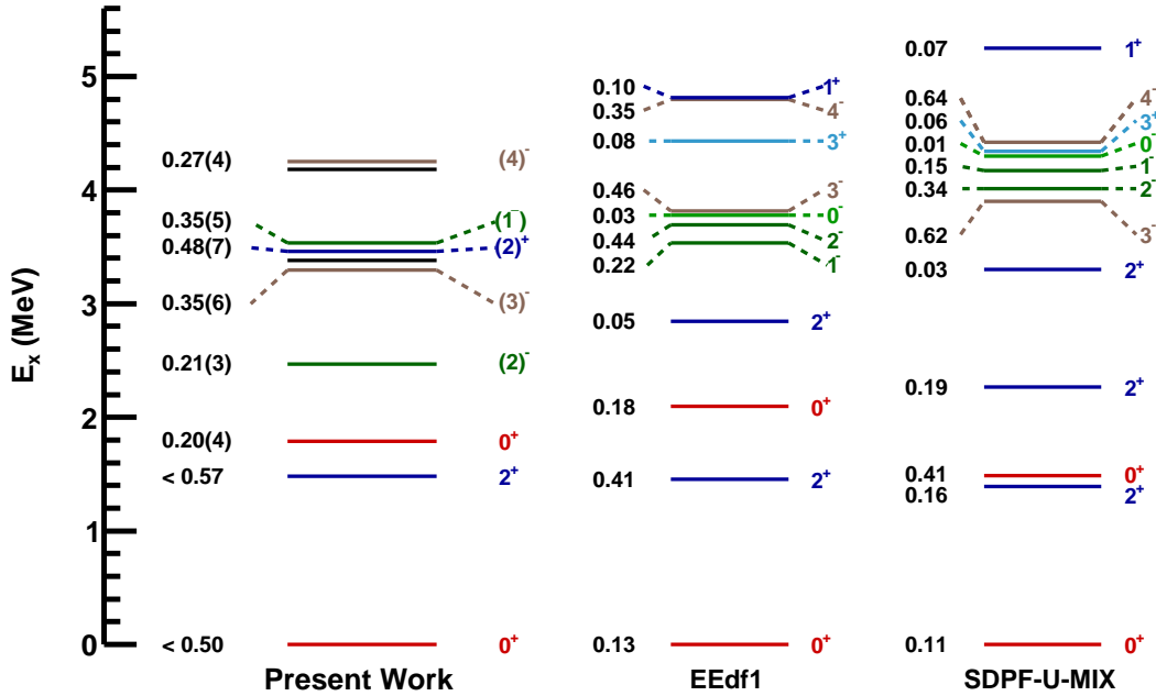
Figure 5: (Color online) Level scheme for ^{30}\text{Mg} obtained in the present work compared to shell model calculations using the EEdf1 [22] and SDPF-U-MIX [15] interactions. Spectroscopic factors (see text and Table 1) and proposed spin-parity assignments are shown on the left and right side of the energy levels, respectively. The orbital angular momentum ( \ell ) for the removed neutron is also indicated: \ell=0 (red), 1 (green), 2 (blue), 3 (brown), undetermined (black) - see Table 1.
