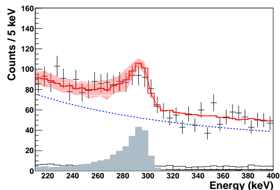
Figure 2: (Color online) Spectrum for the forward angle EXOGAM detectors for E_\gamma < 500 keV. The grey histogram is the simulated lineshape for the 0_2^+ \rightarrow 2_1^+ decay – E_\gamma = 300 \pm 5 keV. The red shading reflects the uncertainty in the half-life – 3.9 \pm 0.5 ns [19].
