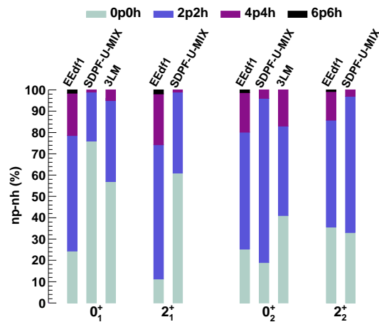
Figure 6: (Color online) Decomposition of the wavefunctions in ^{30}\text{Mg} for the 0_{1,2}^+ and 2_{1,2}^+ states as derived from shell-model calculations employing the EEdf1 and SDPF-U-MIX interactions and, for the 0_{1,2}^+ levels, by a three-level mixing model (3LM) – see text.
