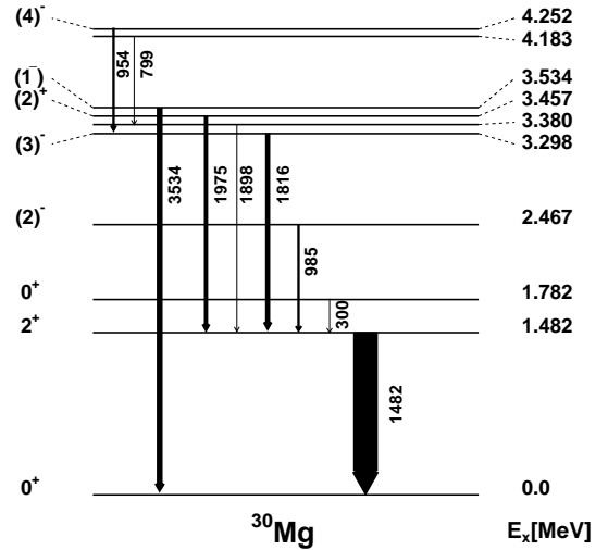
Figure 3: Level scheme of ^{30}\text{Mg} obtained in the present work. The widths of the arrows reflect the absolute intensities of the transitions. The spin-parity assignments above 2 MeV are those deduced here (see text and Table 1).
