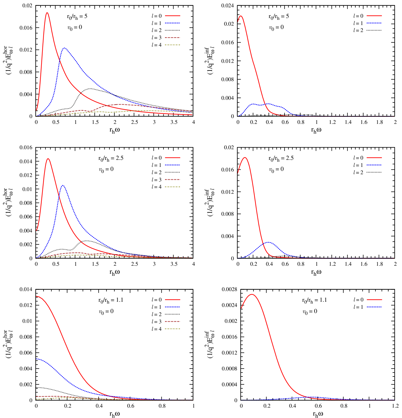
Fig. 3 Numerical estimates of the spectra of the emitted energy, E_{\omega l}^{hor} (plots on the left) and E_{\omega l}^{inf} (plots on the right), as functions of \omega , for selected values of the multipole number, obtained from Eqs. (35)
