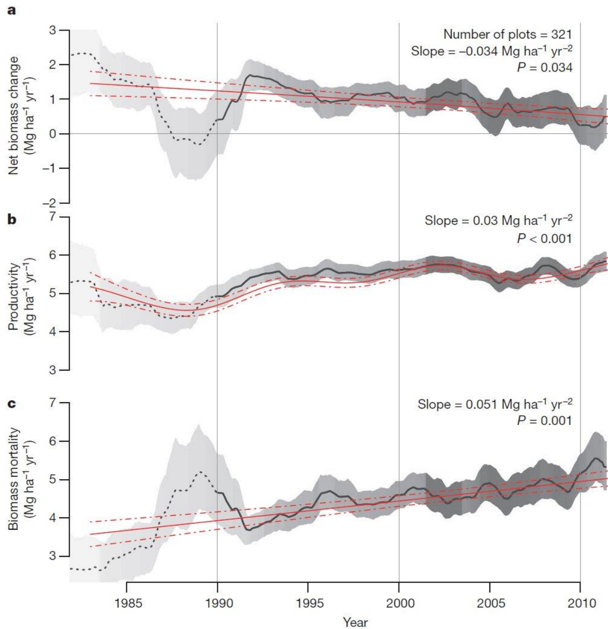
1153 Figure 3. Trends in net above-ground biomass change, productivity and mortality rates, for 1154 321 plots, weighted by plot size (after Brien et al. 2015).
