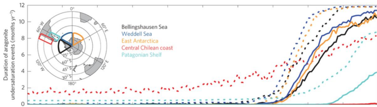
Figure 4. Area-weighted ensemble mean duration (months per year) of aragonite undersaturation at the surface (solid lines) and at 100m depth (dashed lines) for three sectors of the Southern Ocean (Bellingshausen Sea, Weddell Sea and East Antarctica), the central Chilean coast and the Patagonian shelf over the period 1900-2100, with future projections based on RCP 8.5. From Hauri et al. (2016).
