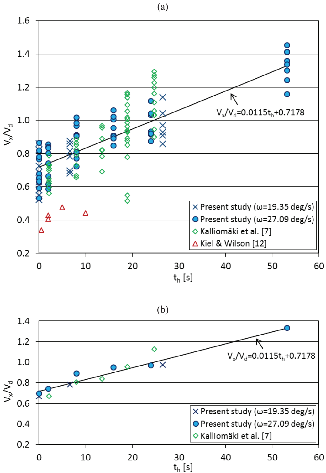
Fig. 9. Normalised exchange volume against hold open time. (a) All data, (b) averages for each hold open time. (All values full scale).
