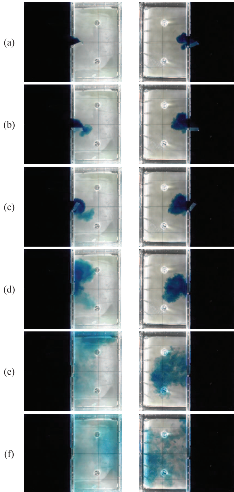
Fig. 4. Time evolution of the exchange flow induced by the door motion (bottom view) for door speed 27.09 deg/s and hold open time 1.99 s. The left column shows the mass flux from Room 1 to Room 2, while the right column shows the mass flux from Room 2 to Room 1. The frames shown are (a) 2.52 s, (b) 5.18 s, (c) 7.17 s, (d) 14.48 s, (e) 55.64 s, (f) 234.92 s after the initiation of the door motion. (All values full scale).
