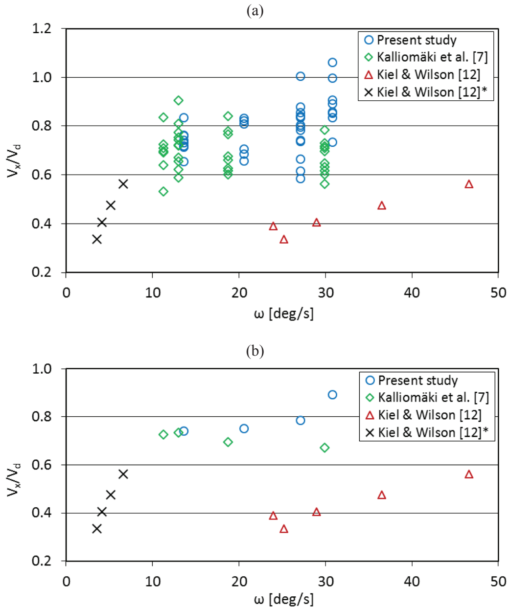
Fig. 10. Normalised exchange volume against angular door speed for a certain hold open time ( t_h=1.99 s for present study, 2.0 s for [7], and 1.0 s for [12]). (a) All data and (b) average data. * Results adapted using Reynolds number similarity (see Table 2). (All values full scale.)
