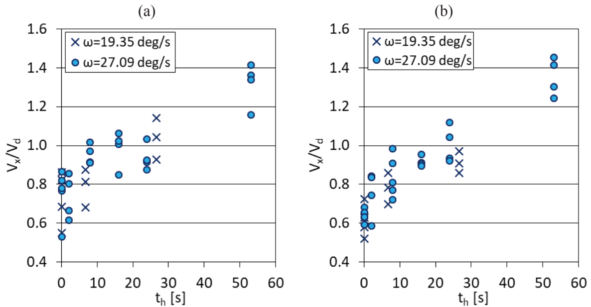
Fig. 8. Normalised exchange volume obtained from (a) Eq. (4a) and (b) Eq. (4b), for two different door speeds and for various hold open times (All values full scale).
