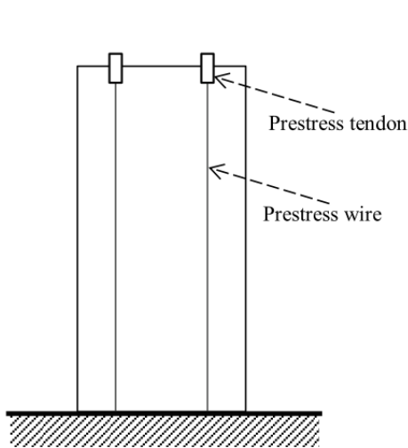
Figure 23 Schematic illustration of post-tensioned timber shear wall
