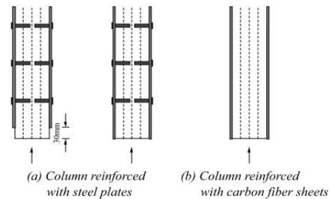
Figure 13 Different reinforcement arrangements [6]
