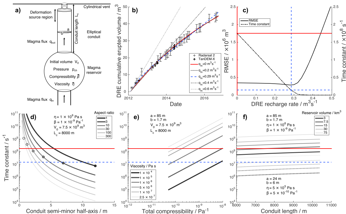
Figure 8. (a) Schematic representation of the magma reservoir used in the models, including the source region for the deformation signal discussed in section 4. (b) Relative fit of different models with constant recharge rates to the lava extrusion observations. (c) Misfit plot, showing the root-mean-square error (RMSE) of models with different constant recharge rate (solid black line) and the trade-off between recharge rate and time constant (dash-dotted black line). In all plots the solid red lines indicate the observed time constant ( \sim 2,000 days) assuming there is no magma recharge ( q_{in} = 0 ), and the dashed blue lines give the best fitting time constant ( \sim 170 days) assuming magma recharge at a constant rate ( q_{in} = 0.29 m^3 s^{-1} ). Plots of t_c dependence on reservoir parameters: (d) conduit cross-section dimensions and aspect ratio, (e) compressibility and magma viscosity, and (f) conduit length and reservoir volume. In each plot, all other parameters are kept constant at the given values. In Figure 8f, the solid lines are plotted using the parameters given for a closed system, while the dotted lines are using the given open system parameters. The filled circles in Figure 8d give the value of b and t_c at given aspect ratios assuming the conduit cross-sectional area is equal to that of the lava spine observed on 28 September 2014.
